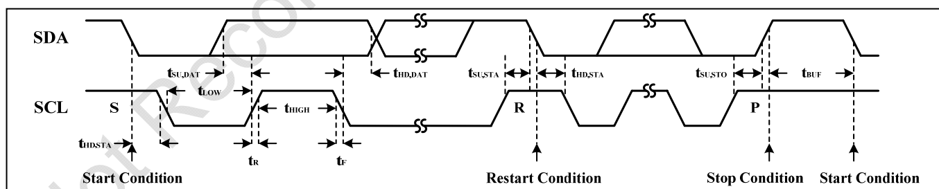
Figure 2 Interface timing
