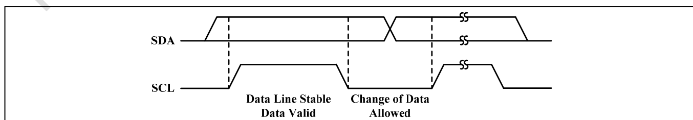
Figure 3 Bit transfer
