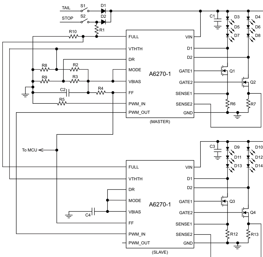
Typical Application Circuit C1: Master-Slave Operation with Internal Reference to DR on Master and MODE Pulled High
