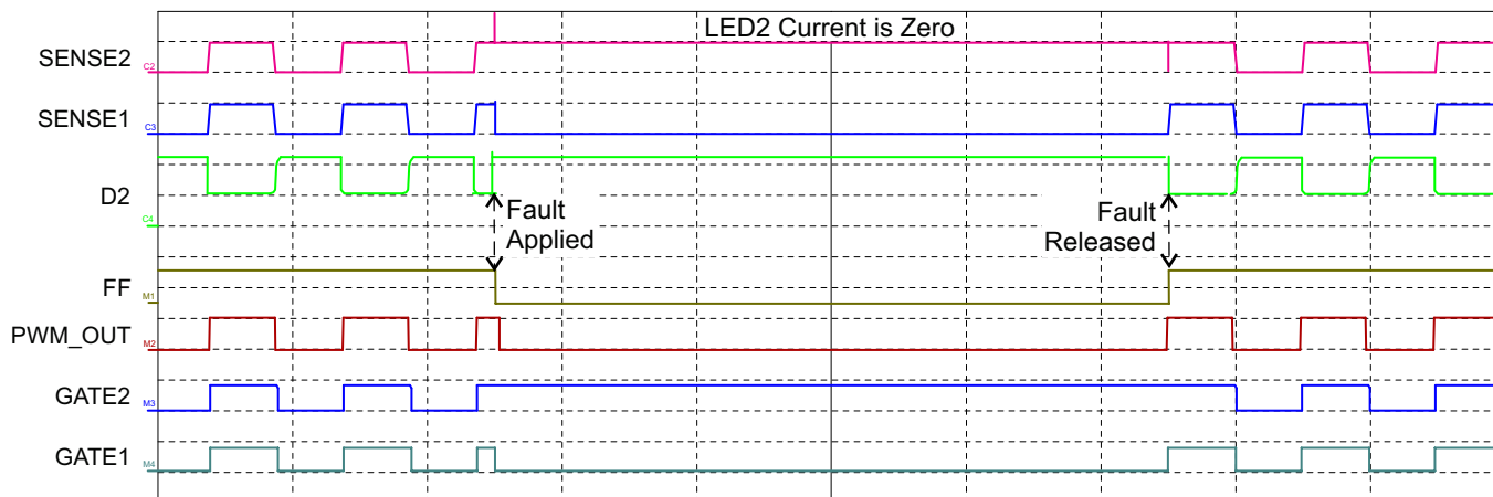
Figure 2a: Drain Short to VIN Fault on D2 with \text{MODE} = \text{HIGH} and PWM Dimming
