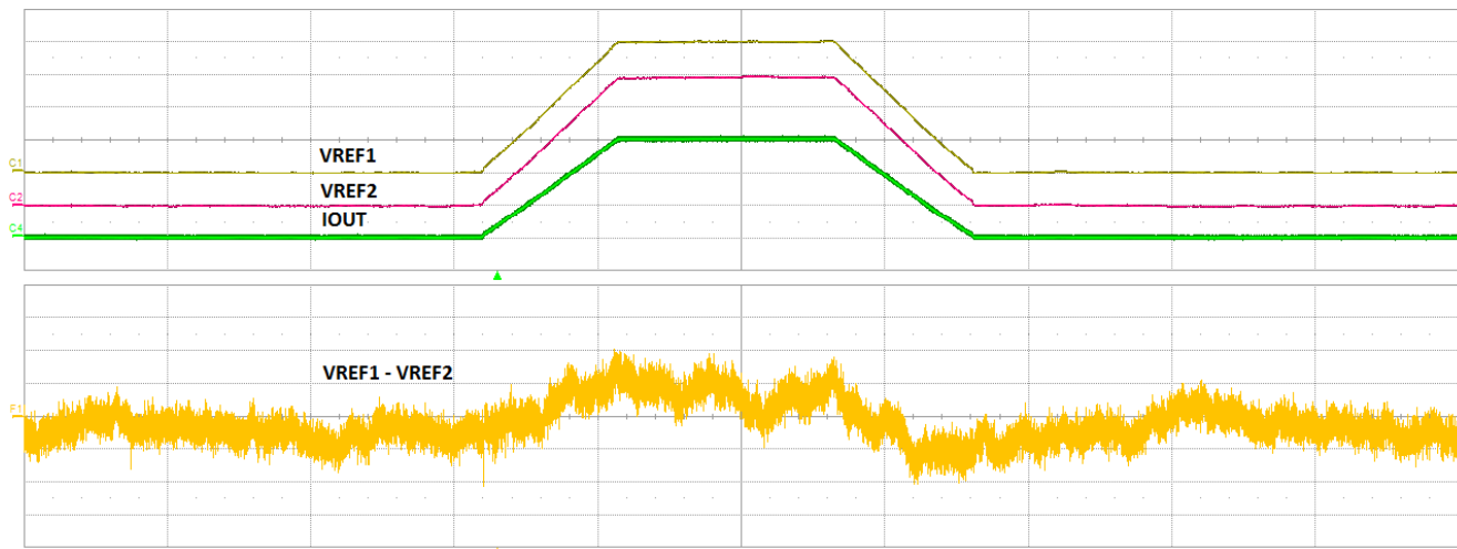
Figure 16: Reference Matching During PWM Dimming V_{REF1} , V_{REF2} (50 mV/div), I_{OUT} (Total LED Current) (200 mA/div), V_{REF1} - V_{REF2} (2 mV/div), Time (100 \mu s/div).
