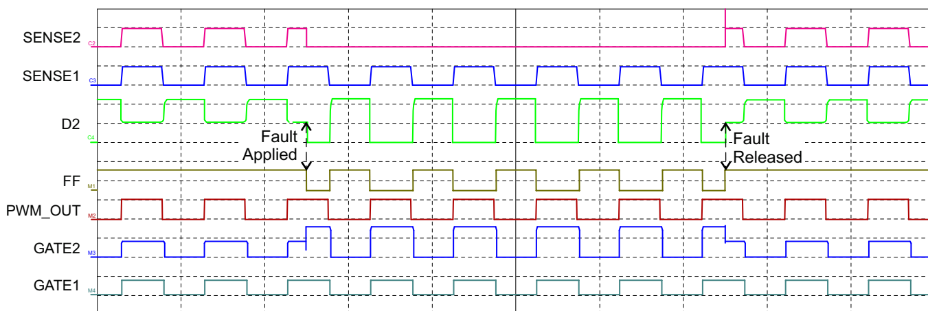
Figure 4b: Open LED Fault on D2 with MODE = LOW and PWM Dimming
