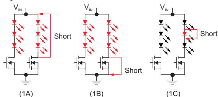
Figure 1: Short-Circuit Protection
