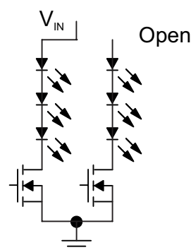
Figure 3: LED Open Protection
