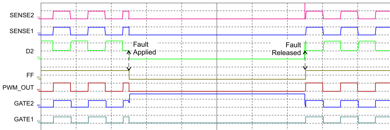
Figure 4a: Open LED Fault on D2 with MODE = HIGH and PWM Dimming
