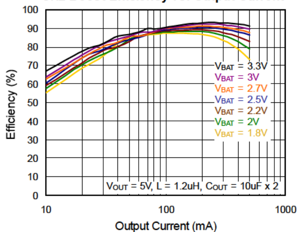
CH2 Boost Efficiency vs. Output Current
