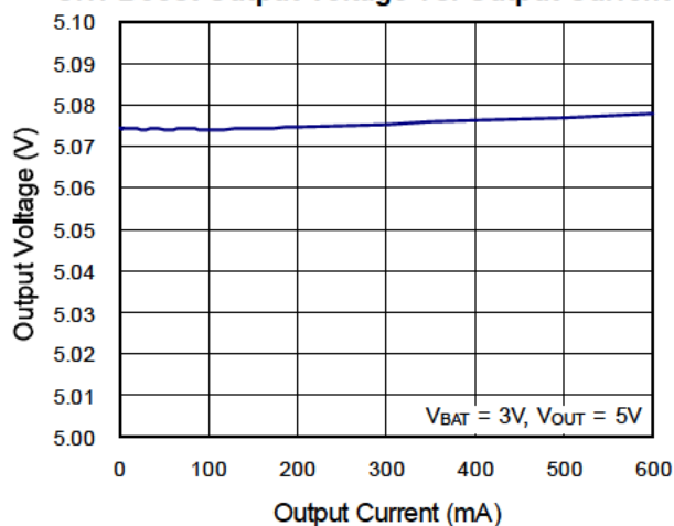
CH1 Boost Output Voltage vs. Output Current
