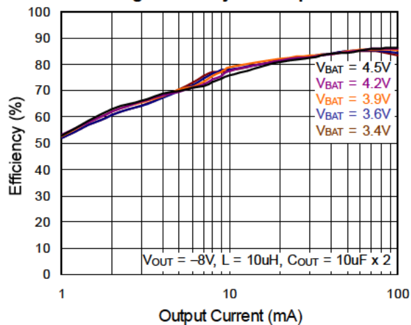
CH6 Inverting Efficiency vs. Output Current
