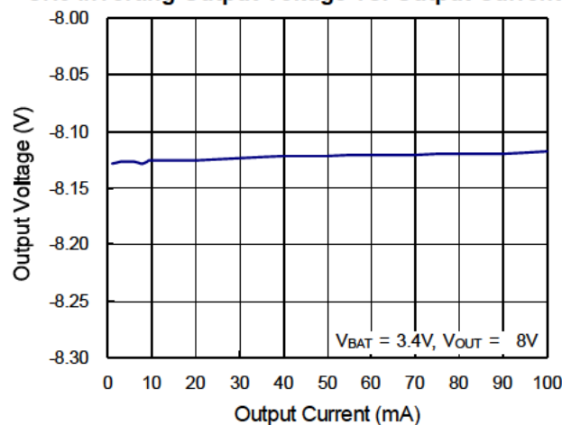
CH6 Inverting Output Voltage vs. Output Current
