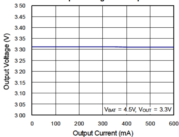
CH2 Buck Output Voltage vs. Output Current
