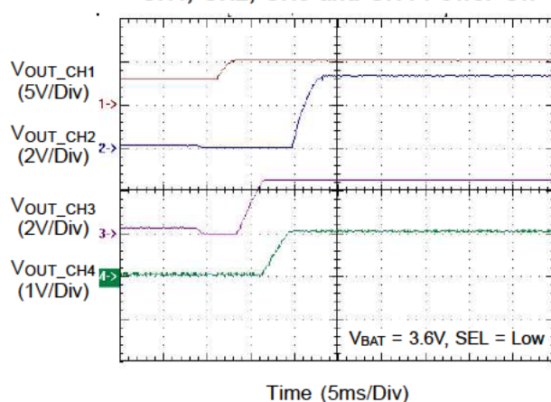
CH1, CH2, CH3 and CH4 Power On
