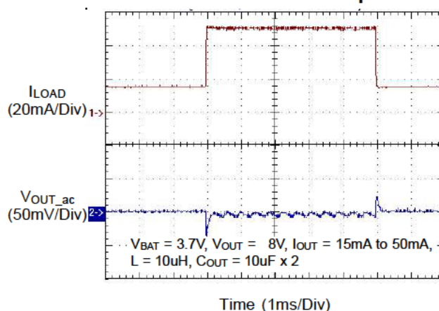
CH6 Load Transient Response
