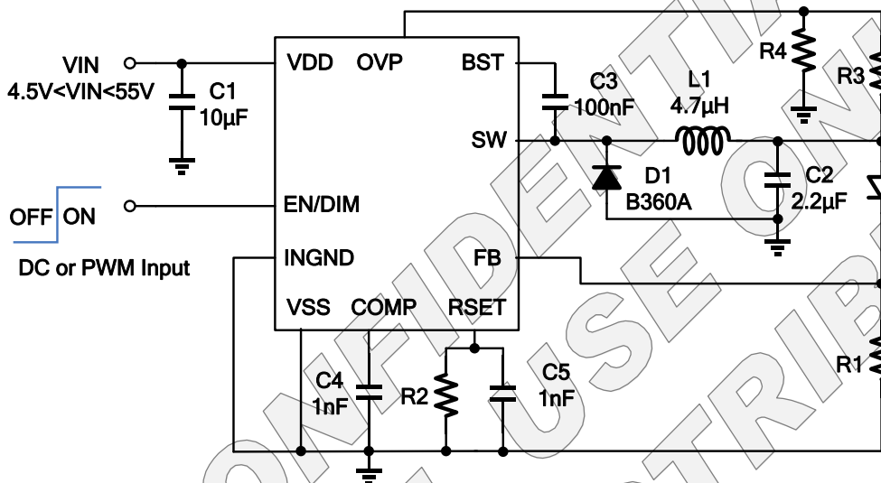
Figure 3—Step-Down White LED Driver Application
