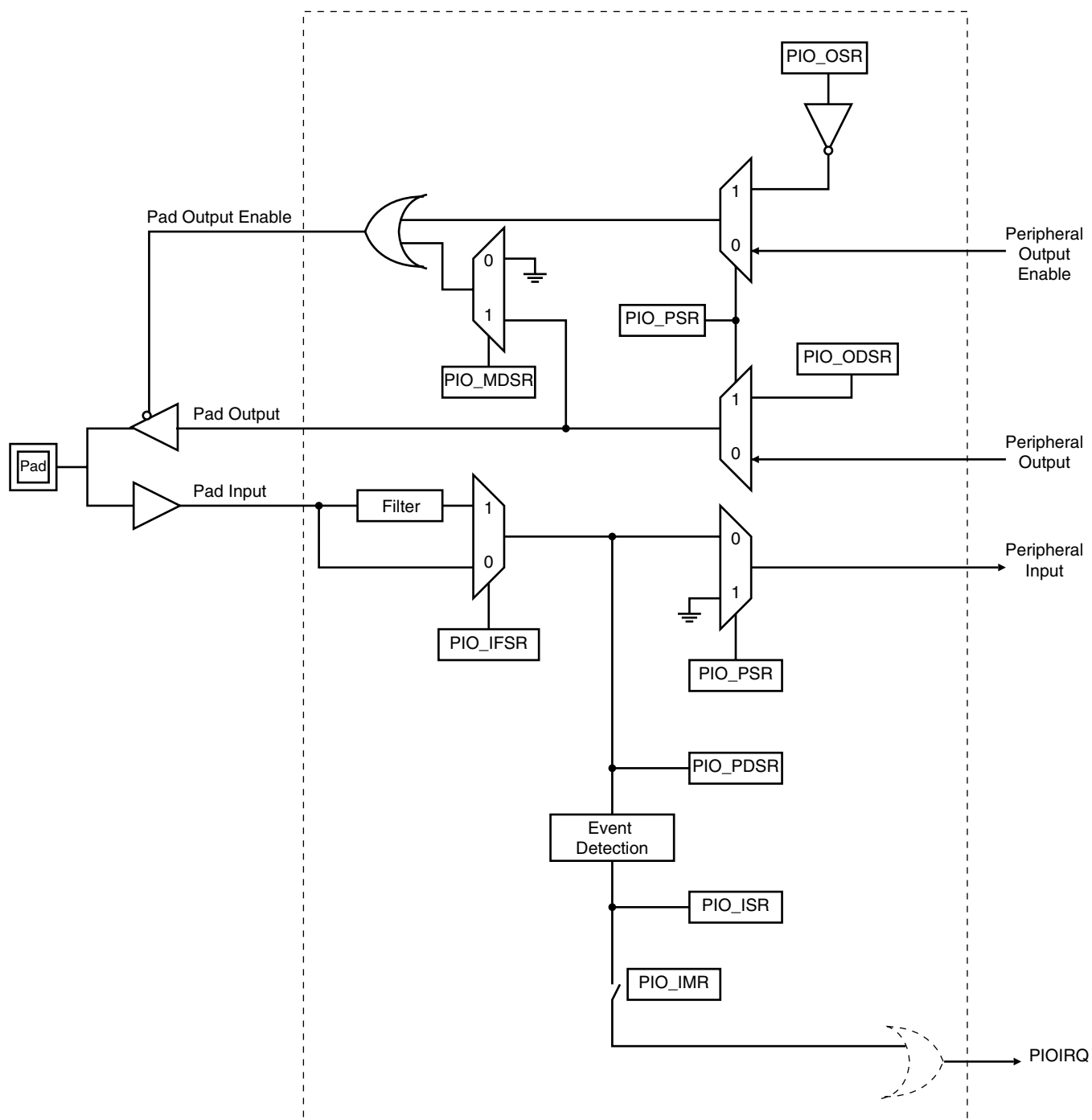
Figure 38. Parallel I/O Multiplexed with a Bi-directional Signal
