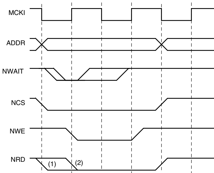
Figure 19. External Wait
