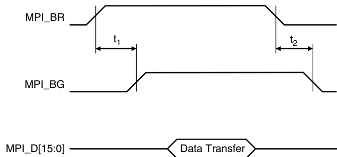
Figure 35. External Arbitration
