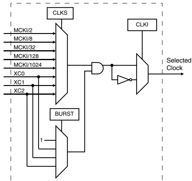
Figure 54. Clock Selection
