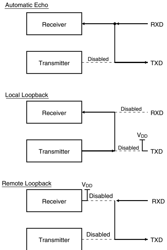
Figure 45. Channel Modes
