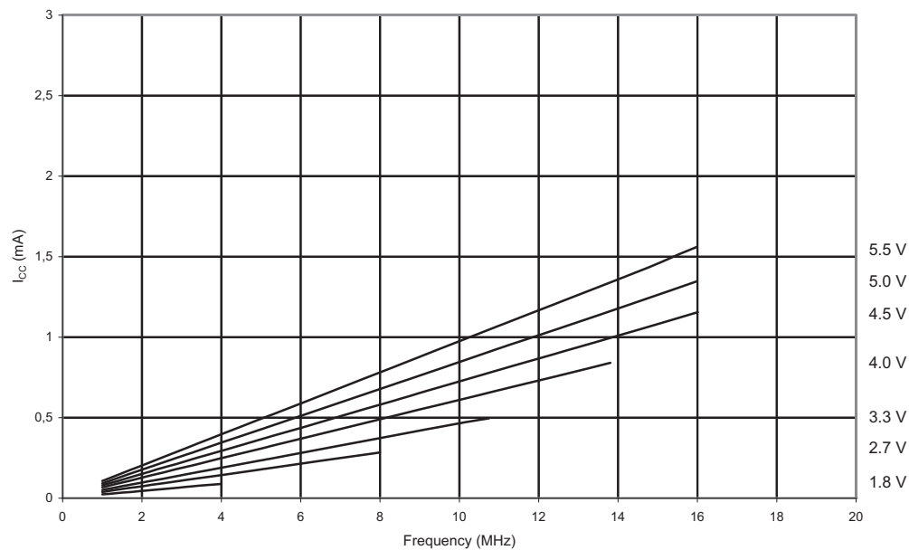
Figure 3-103.Reset Supply Current vs. V_{CC} 1 - 16 MHz, Excluding Current through Reset Pull-up)
