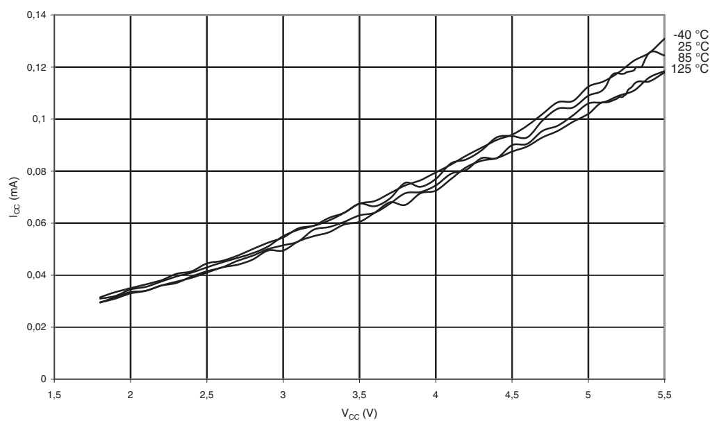
Figure 3-49. Active Supply Current vs. V_{CC} (Internal RC Oscillator, 128 kHz)
