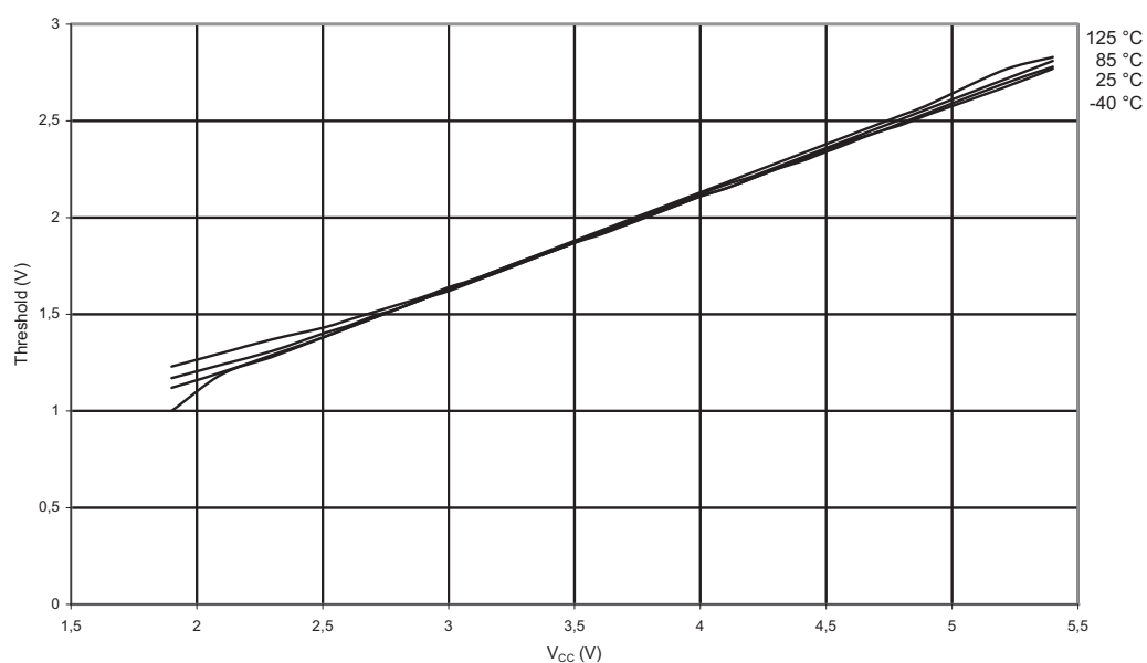
Figure 3-123. V_{IH} : Input Threshold Voltage vs. V_{CC} (Reset Pin as I/O, Read as '1')
