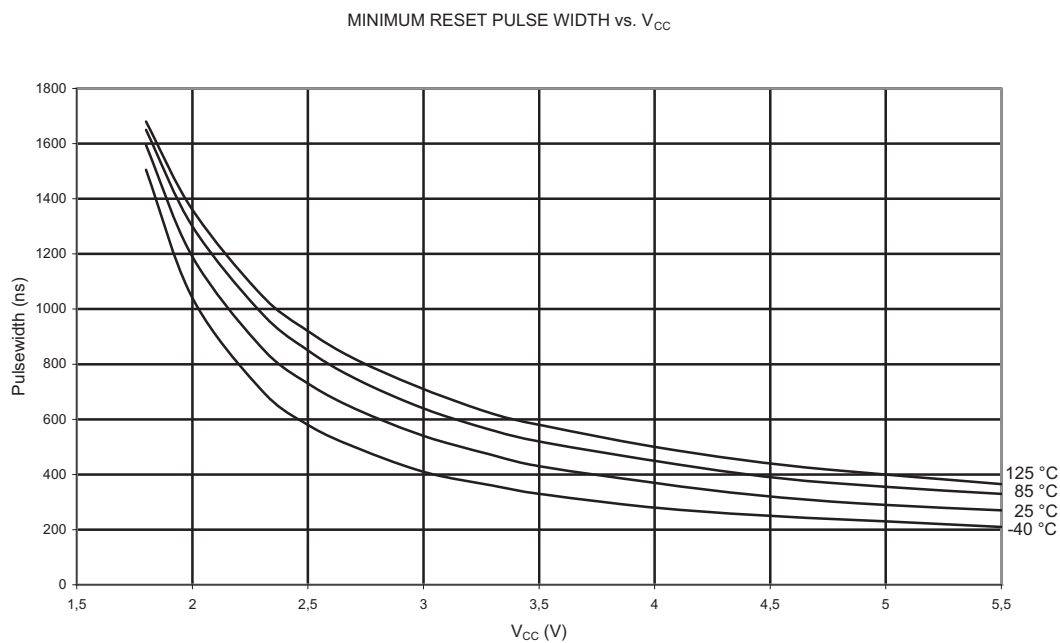
Figure 3-41. Minimum Reset Pulse Width vs. V_{CC}
