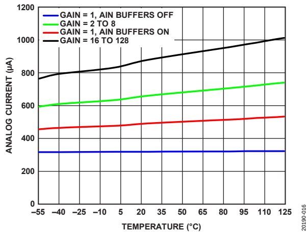
Figure 16. Analog Current vs. Temperature (Full Power Mode)
