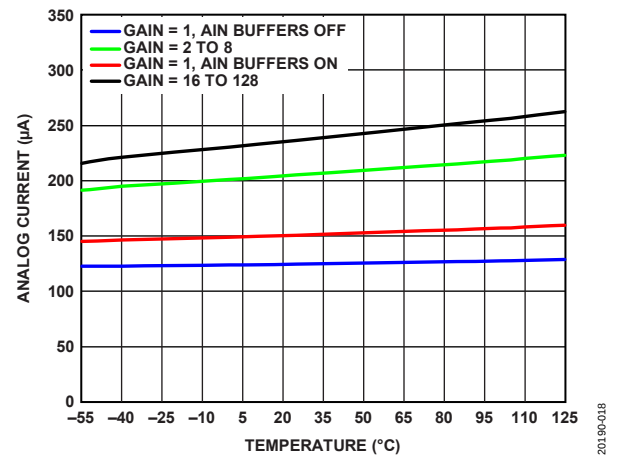
Figure 18. Analog Current vs. Temperature (Low Power Mode)
