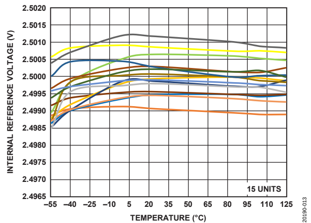
Figure 13. Internal Reference Voltage vs. Temperature
