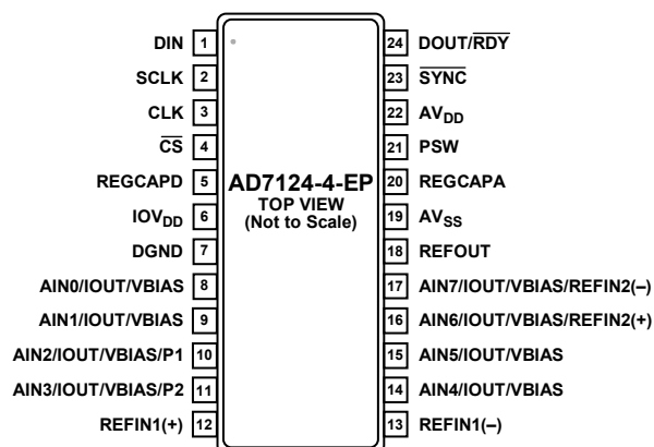
Figure 2. Pin Configuration
