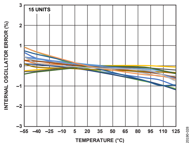
Figure 21. Internal Oscillator Error vs. Temperature
