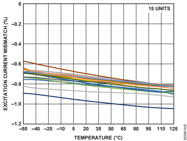
Figure 15. Excitation Current Drift Matching (500 µA)
