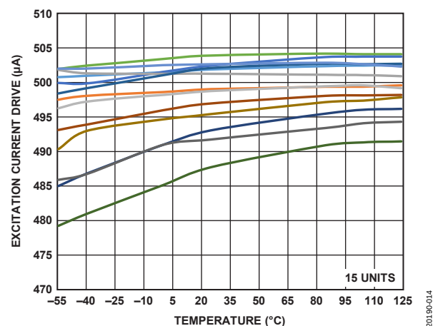
Figure 14. Excitation Current Drift (500 \mu A)
