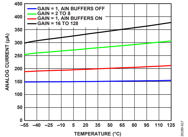
Figure 17. Analog Current vs. Temperature (Mid Power Mode)
