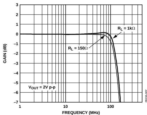
Figure 9. Large Signal Frequency Response at Various Loads
