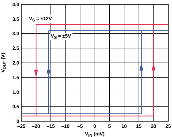
Figure 36. Comparator Hysteresis
