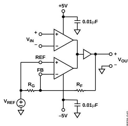
Figure 39. Basic Gain Circuit: V_{OUT} = V_{IN}(1 + R_F/R_G) + V_{REF}
