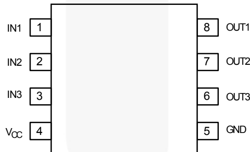
Figure 2. Pin Configuration
