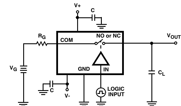
FIGURE 1. SWITCHING TIMES
