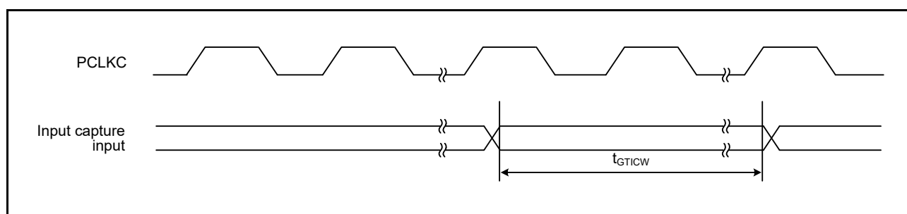
Figure 5.41 GPTW Input Capture Input Timing
