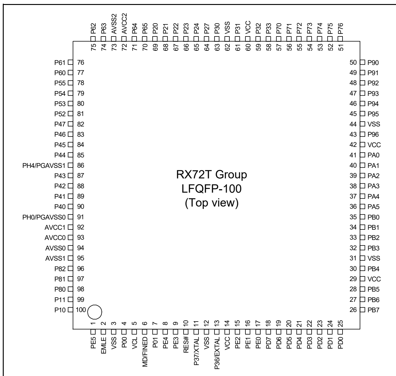
Figure 1.5 Pin Assignment (100-pin LFQFP) with PGA pseudo-differential input and without USB pin
