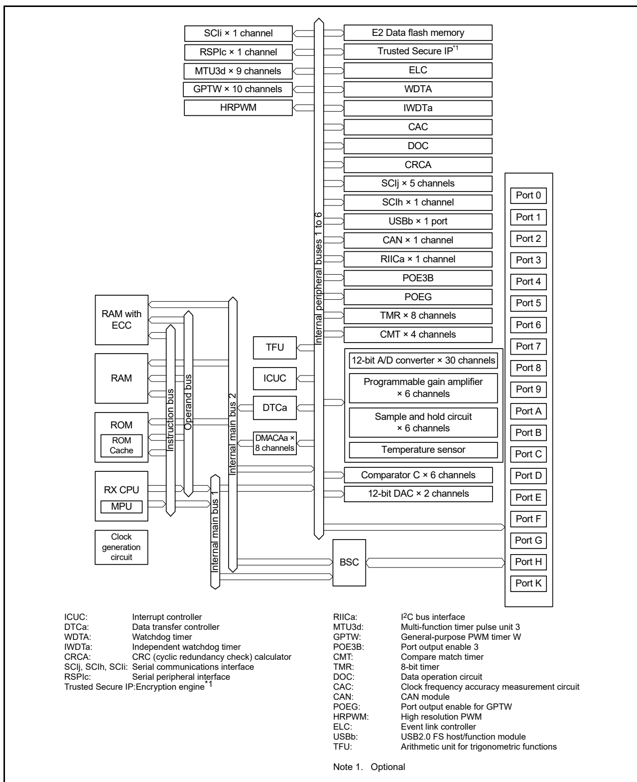
Figure 1.2 Block Diagram
