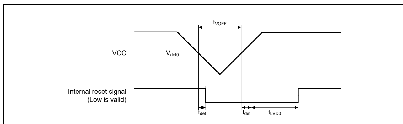
Figure 5.62 Voltage Detection Circuit Timing (V det0 )
