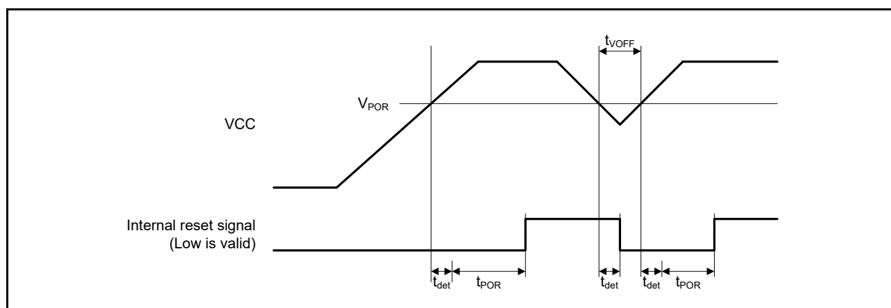
Figure 5.61 Power-on Reset Timing
