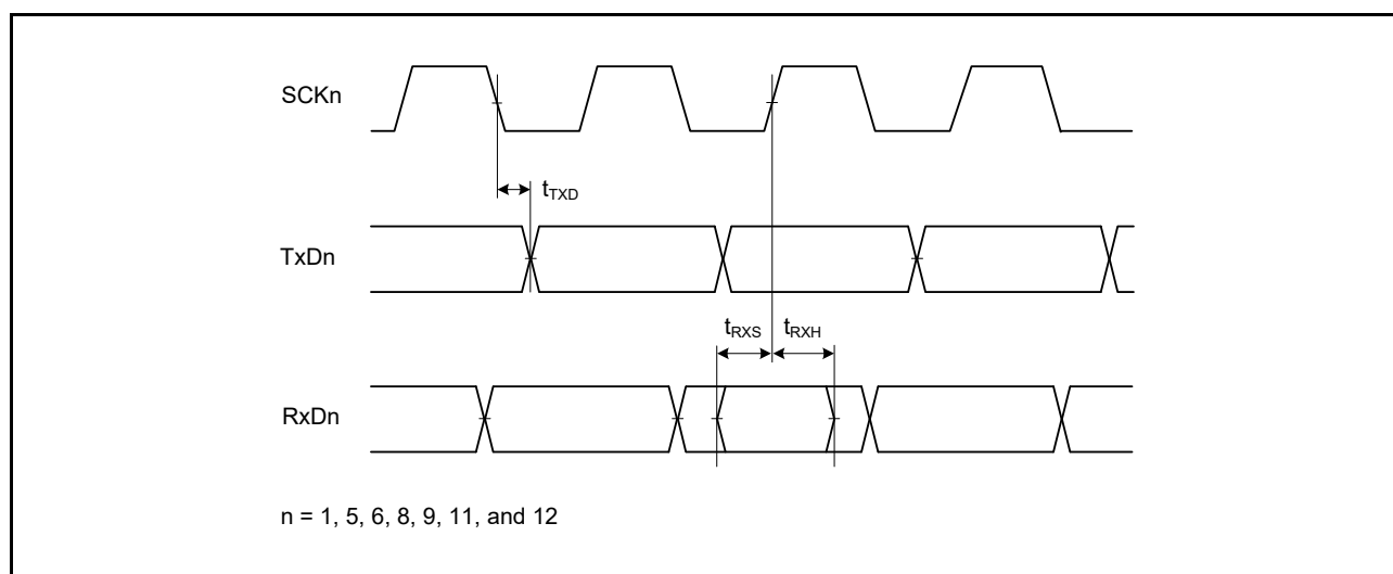
Figure 5.46 SCI Input/Output Timing: Clock Synchronous Mode
