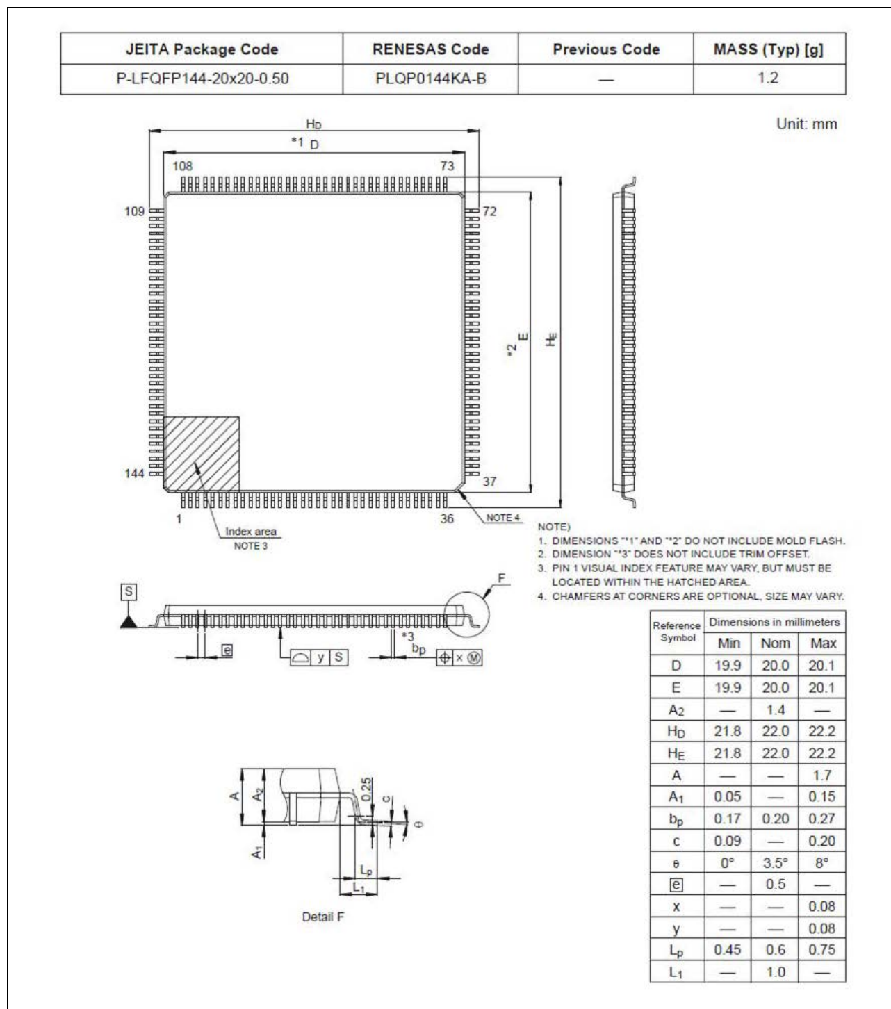
Figure A 144-Pin LFQFP (PLQP0144KA-B)
