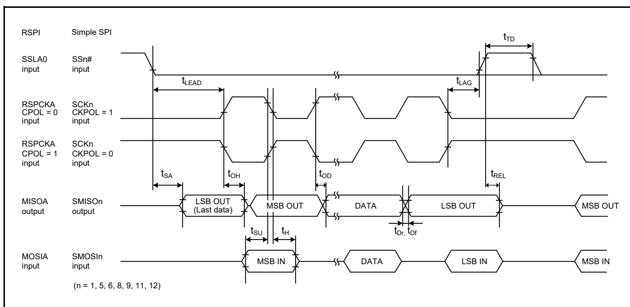
Figure 5.53 RSP Timing (Slave, CPHA = 1) and Simple SPI Timing (Slave, CKPH = 0)
