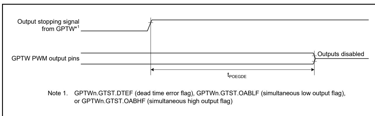
Figure 5.35 Output Disable Time for POEG in Response to Detection of the Output Stopping Signal from GPTW
