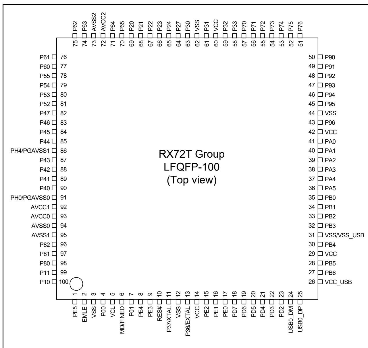
Figure 1.4 Pin Assignment (100-pin LFQFP) with PGA pseudo-differential input and with USB pin
