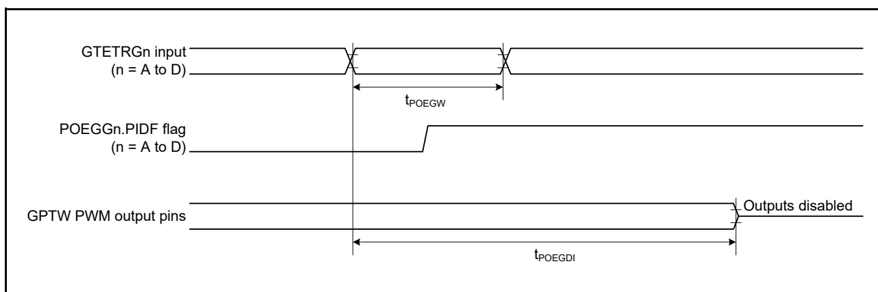
Figure 5.34 Output Disable Time for POEG via Detection Flag in Response to the Input Level Detection of the GTETR Gn pin
