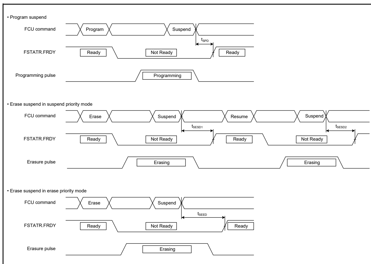
Figure 5.66 Flash Memory Program/Erase Suspend Timing
