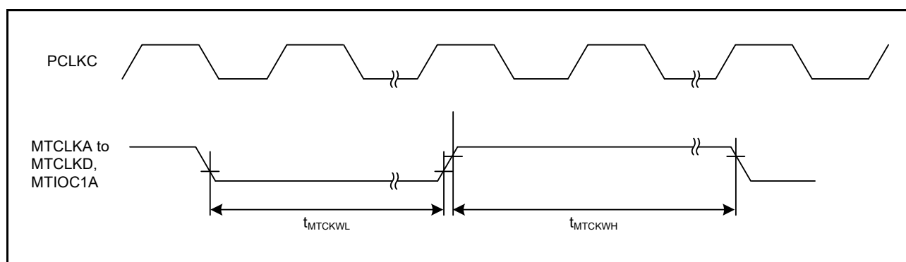
Figure 5.26 MTU Clock Input Timing
