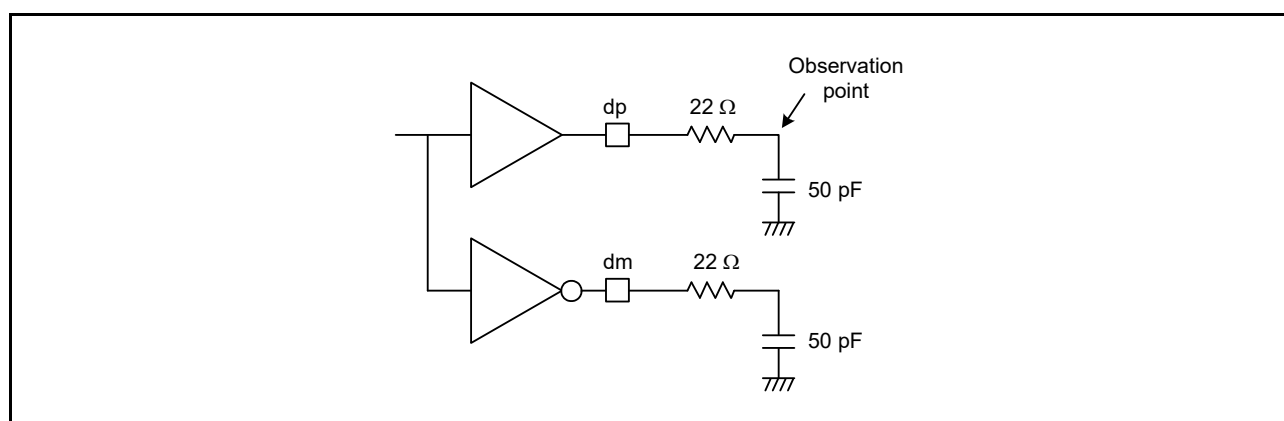
Figure 5.58 Test Circuit (Full-Speed)
