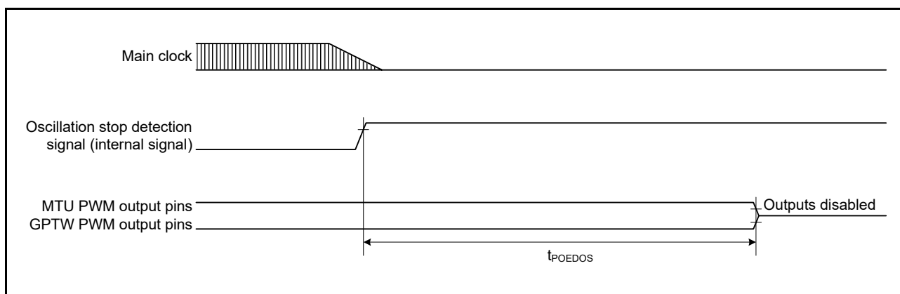
Figure 5.32 Output Disable Time for POE in Response to the Oscillation Stop Detection
