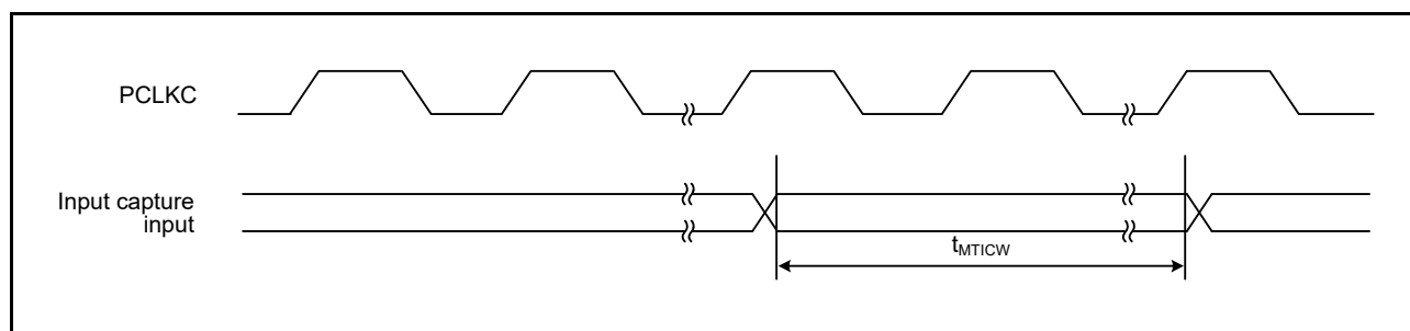
Figure 5.25 MTU Input Capture Input Timing
