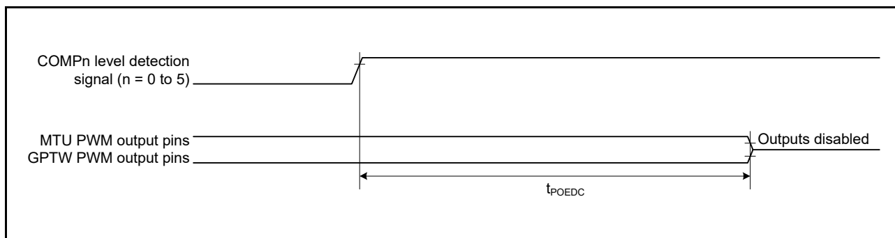
Figure 5.30 Output Disable Time for POE in Response to Detection of the Comparator Outputs
