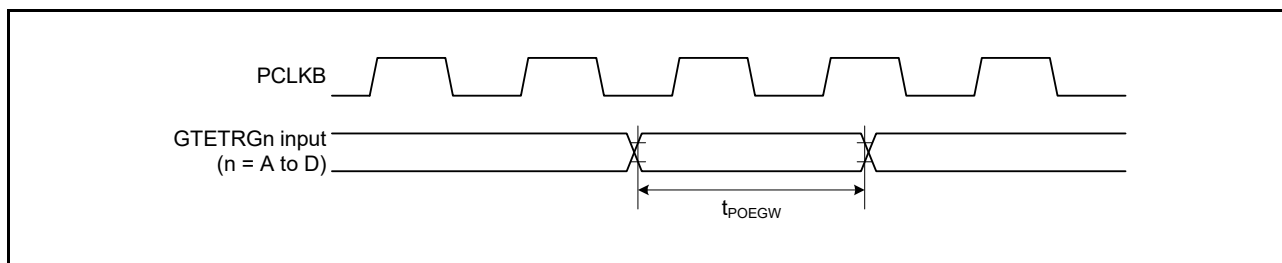
Figure 5.33 POEG Input Timing
