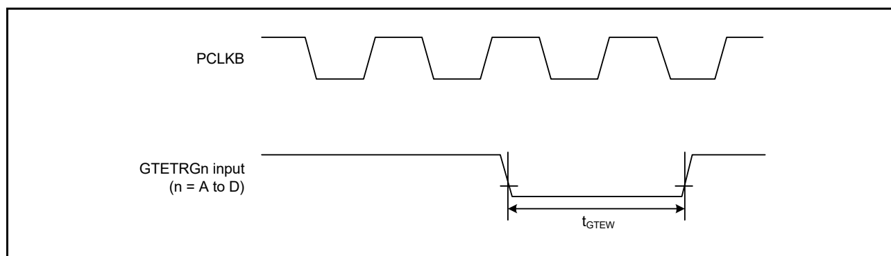
Figure 5.42 GPTW External Trigger Input Timing
