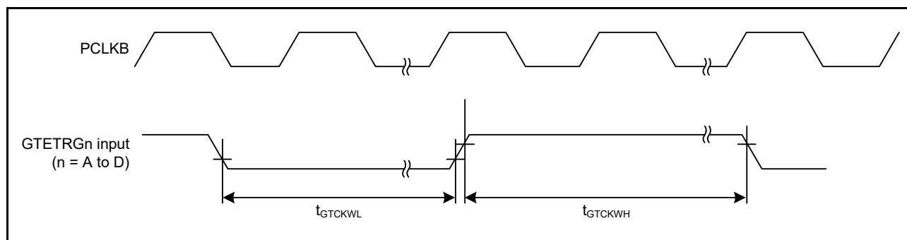
Figure 5.43 GPTW Clock Input Timing
