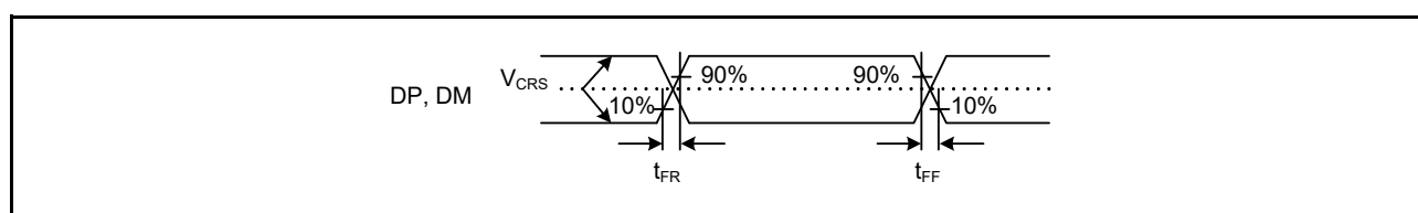
Figure 5.57 DP and DM Output Timing (Full-Speed)
