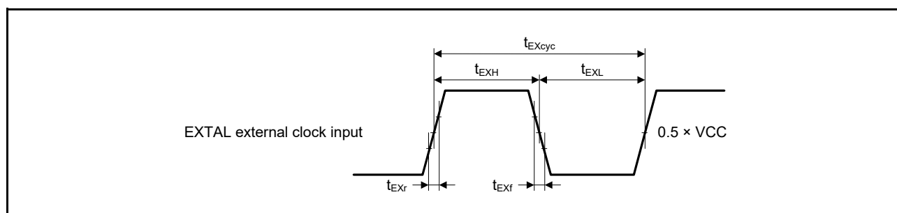
Figure 5.5 EXTAL External Clock Input Timing
