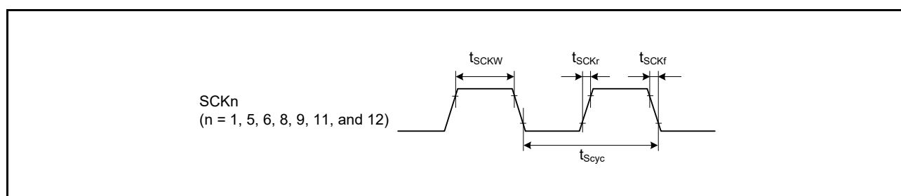
Figure 5.45 SCK Clock Input Timing
