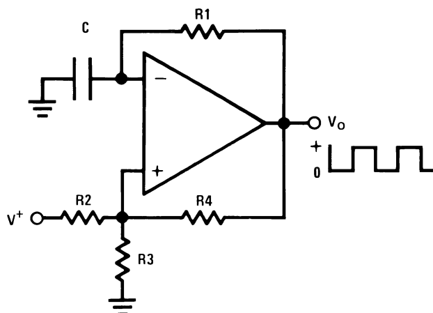
Figure 9-14. Squarewave Generator
