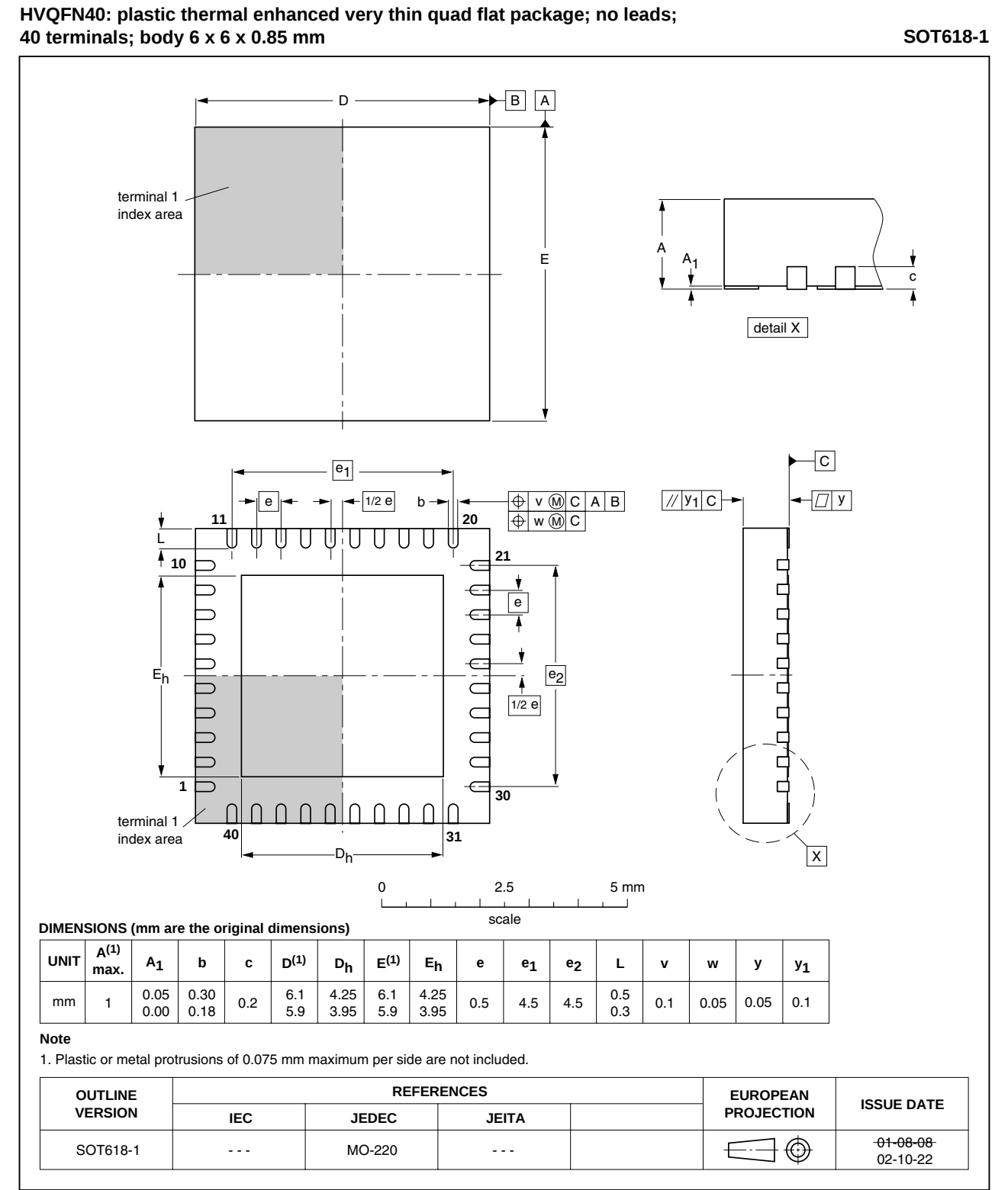
Fig 35. Package outline SOT618-1 (HVQFN40)
