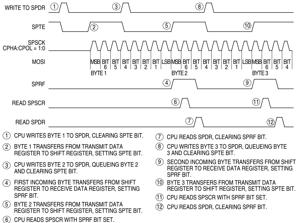
Figure 13-8. SPSCr/SPTe CPU Interrupt Timing
