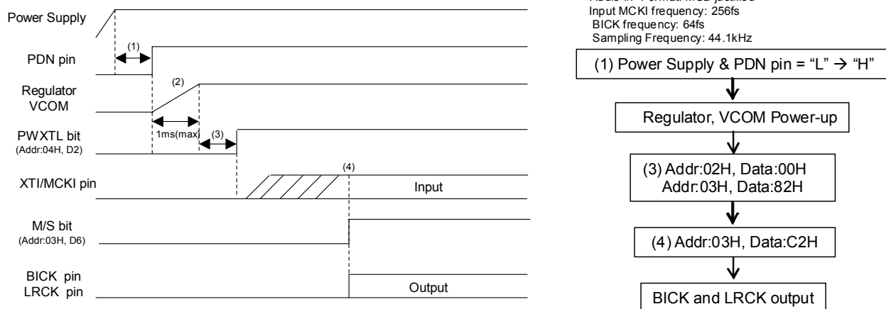
Figure 80. Clock Set Up Sequence (4)
