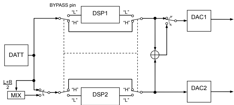
Figure 44. Bypass Mode
