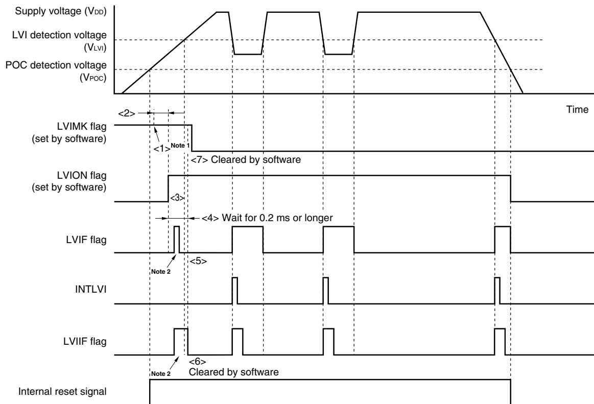
Figure 14-5. Timing of Low-Voltage Detector Interrupt Signal Generation
