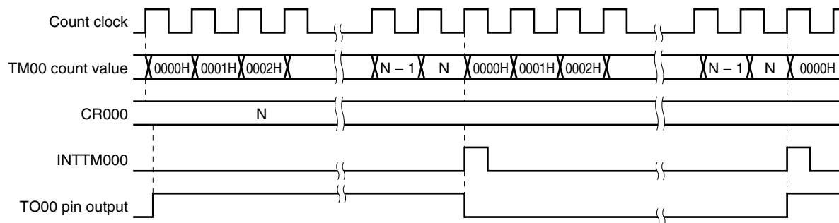
Figure 6-29. Square-Wave Output Operation Timing
