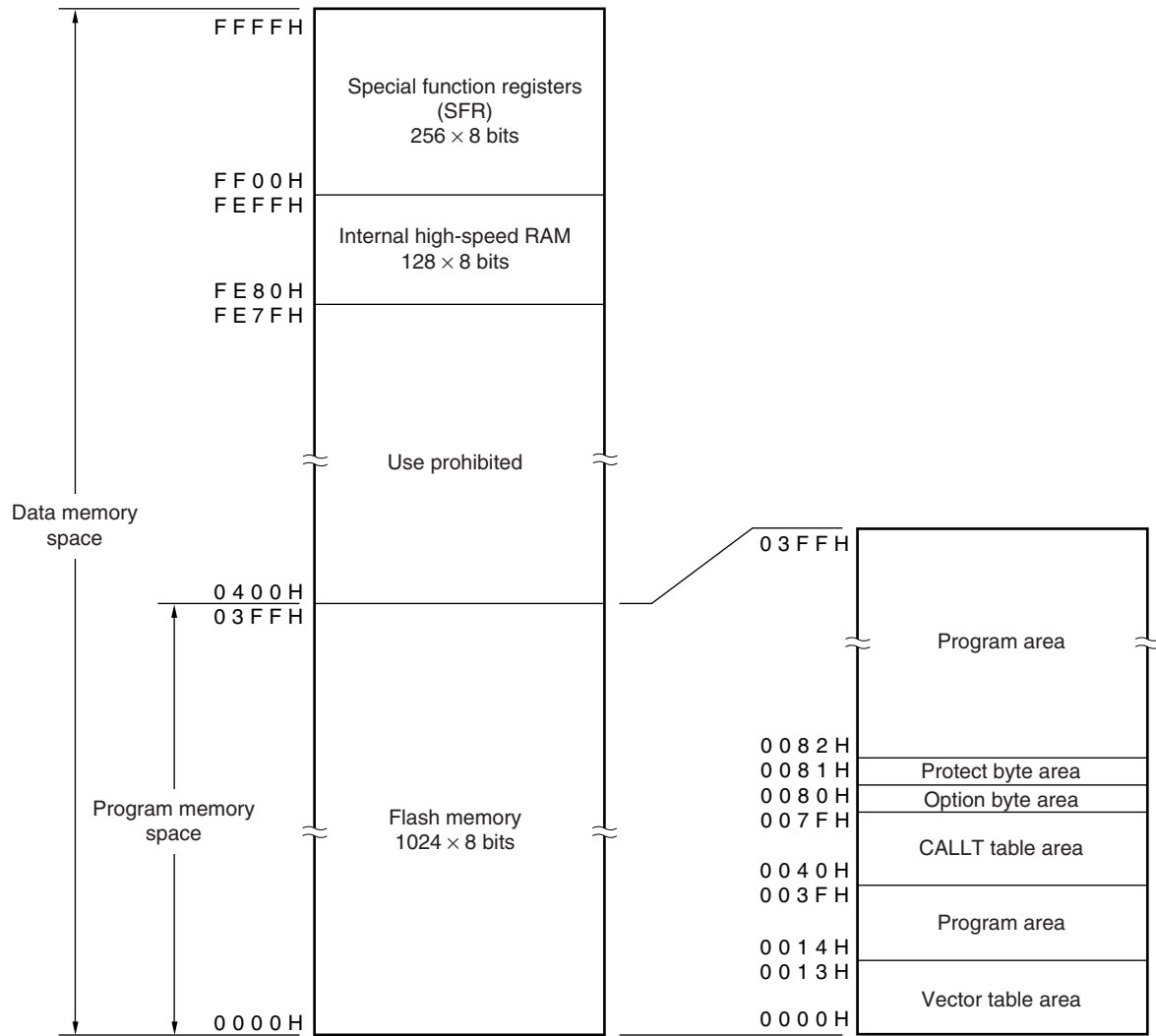
Figure 3-1. Memory Map ( \mu PD78F9200, 78F9210)
