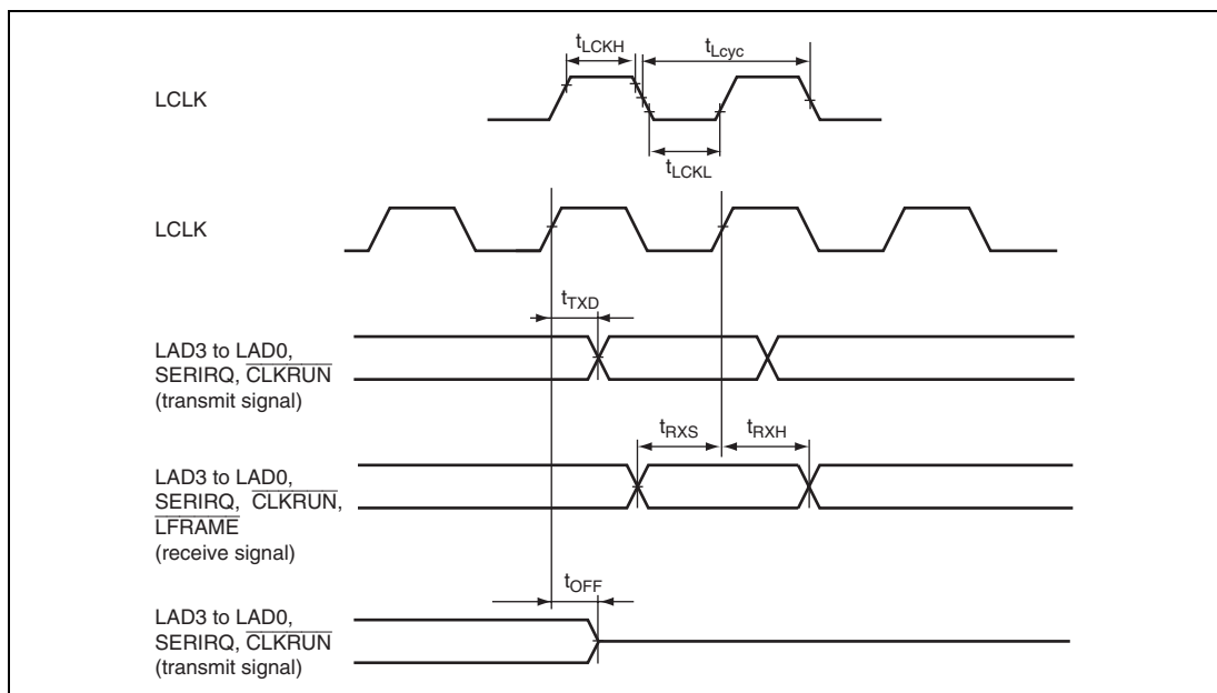
Figure 31.23 LPC Interface (LPC) Timing
