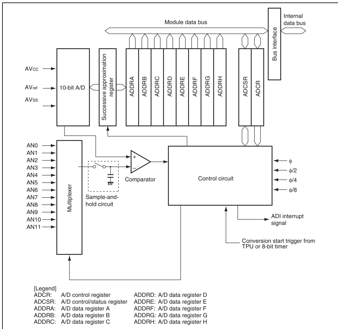
Figure 24.1 Block Diagram of A/D Converter
