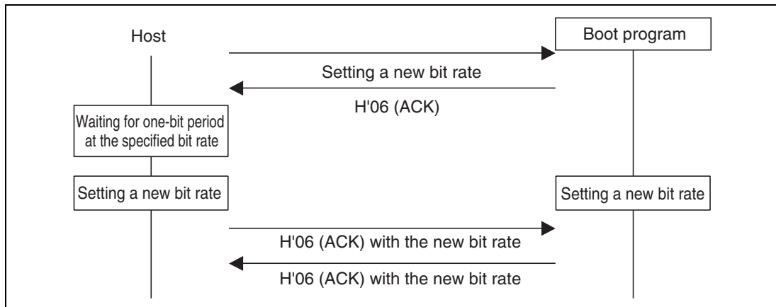
Figure 27.19 New Bit-Rate Selection Sequence
