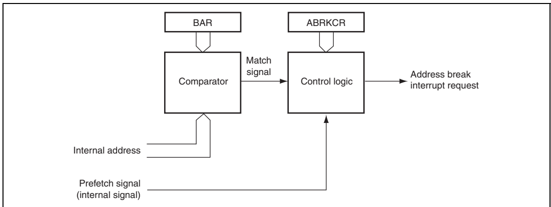
Figure 7.10 Block Diagram of Address Break Function
