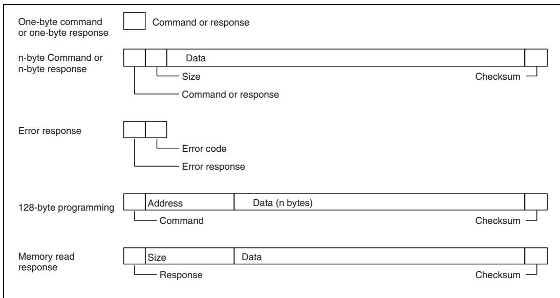
Figure 27.18 Communication Protocol Format
