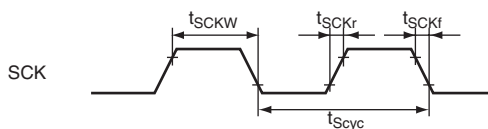
Figure 31.18 SCK Clock Input Timing
