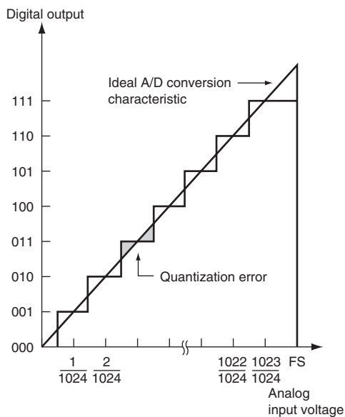
Figure 24.6 A/D Conversion Accuracy Definitions
