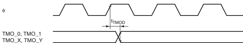
Figure 31.12 8-Bit Timer Output Timing
