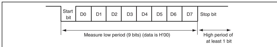
Figure 27.12 Automatic-Bit-Rate Adjustment Operation
