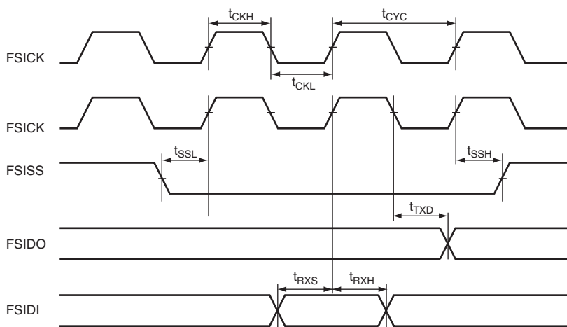
Figure 31.20 FSI Input/Output Timing
