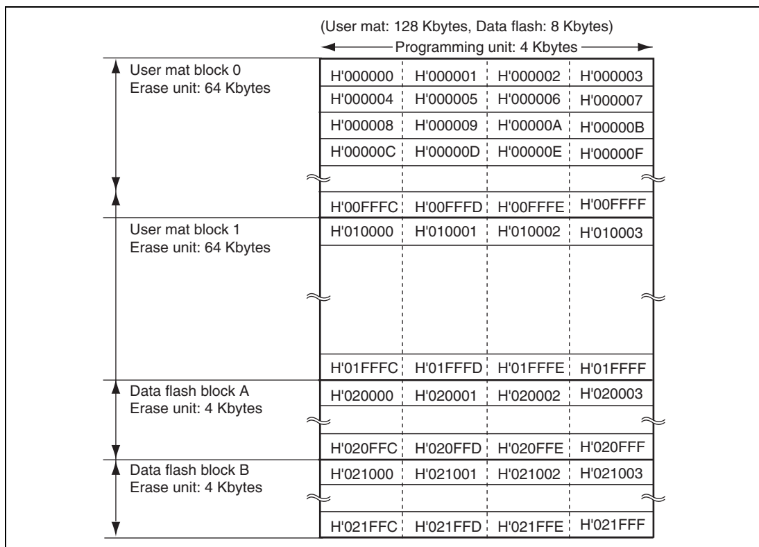
Figure 27.3 Block Structure of Flash Memory
