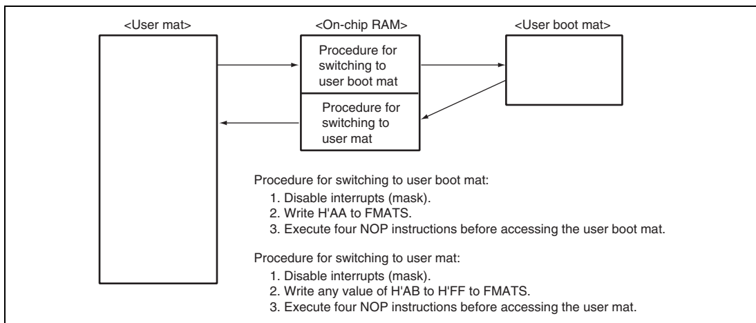
Figure 27.15 Switching between User Mat and User Boot Mat
