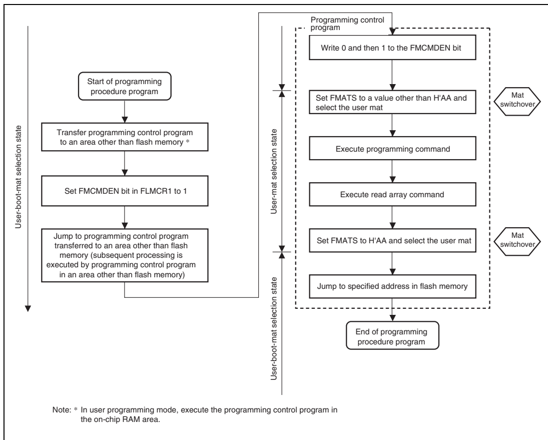
Figure 27.13 Procedure for Programming the User Mat in User Boot Mode
