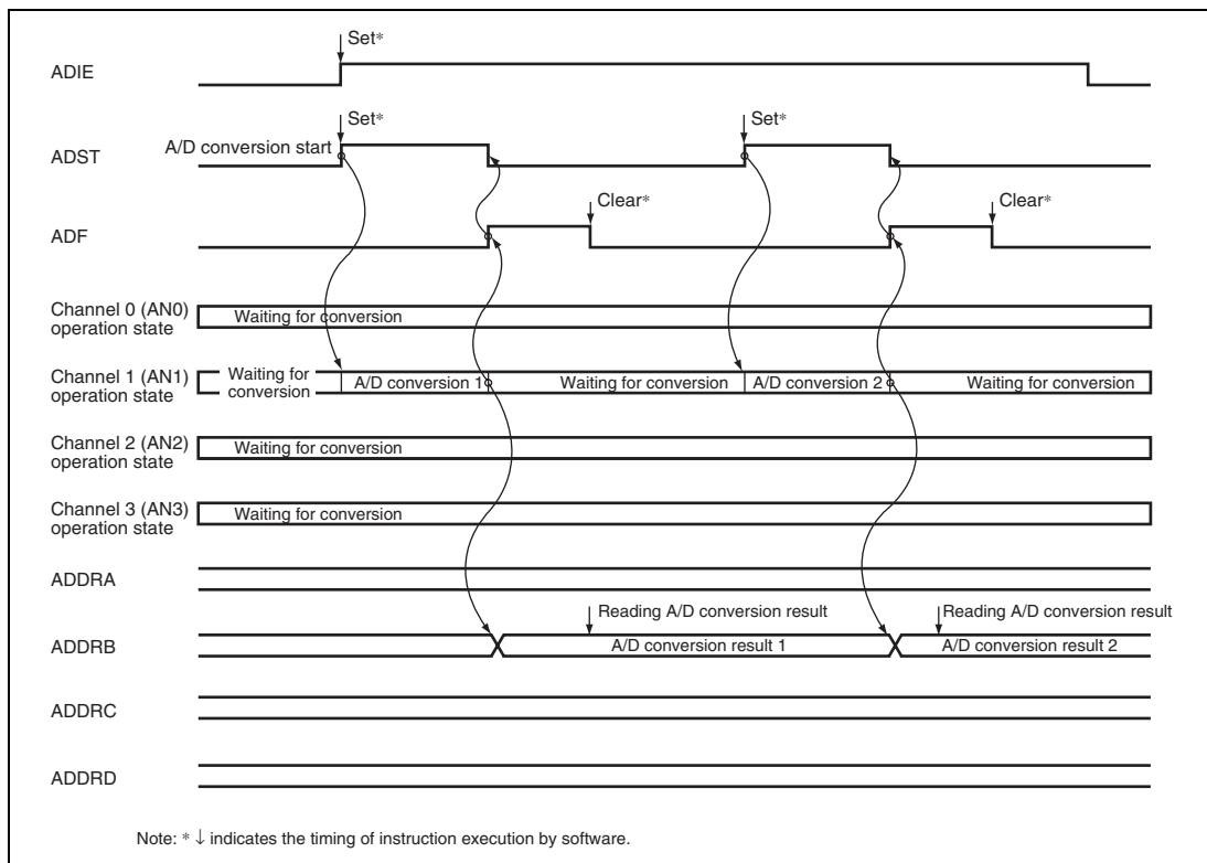
Figure 24.2 Example of A/D Converter Operation (Single Mode, Channel 1 Selected)
