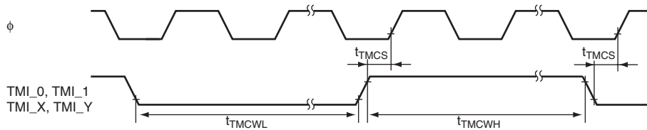
Figure 31.13 8-Bit Timer Clock Input Timing
