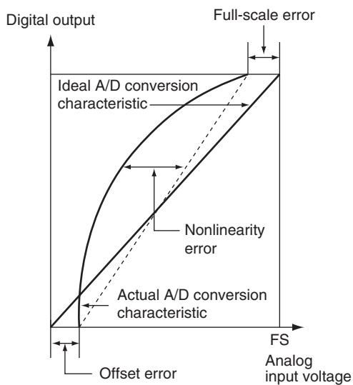
Figure 24.7 A/D Conversion Accuracy Definitions
