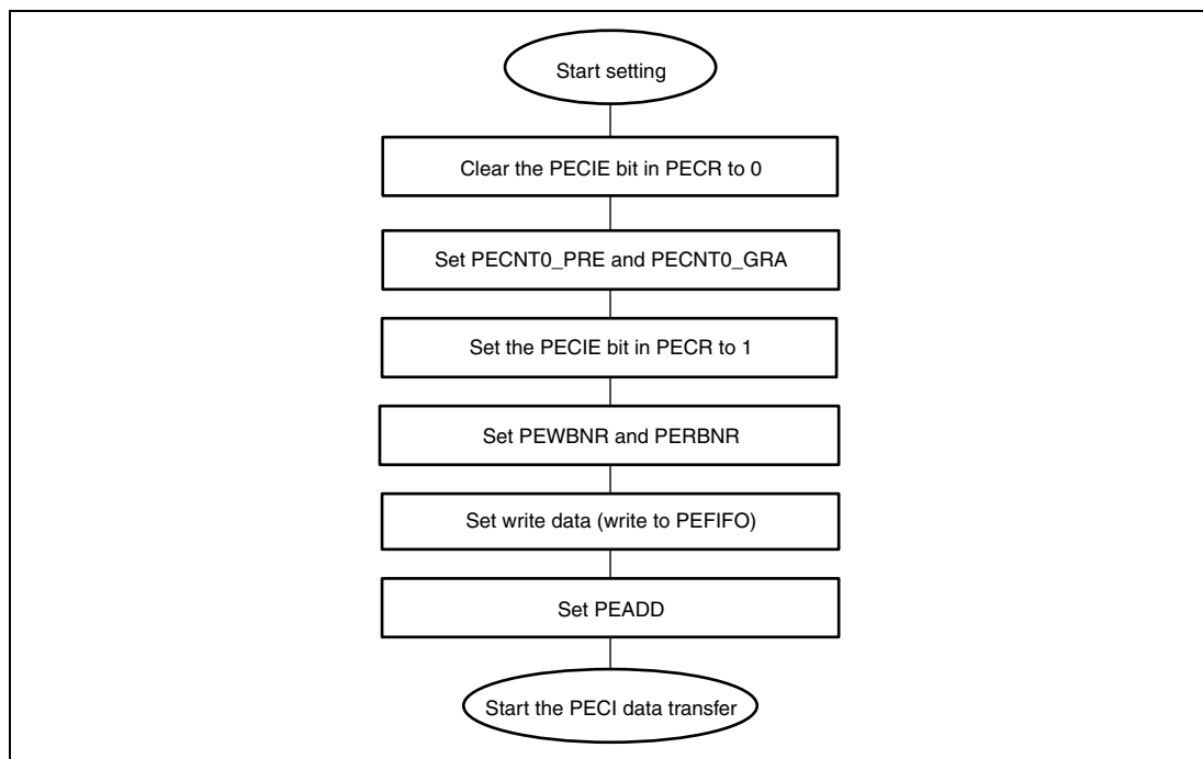
Figure 23.2 Sample Flowchart of Configuring the PECI
