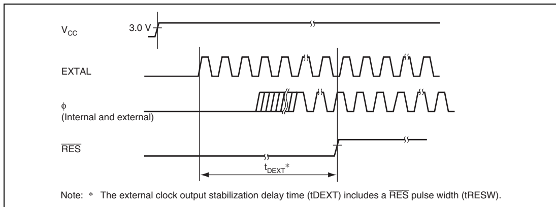
Figure 28.6 Timing of External Clock Output Stabilization Delay Time
