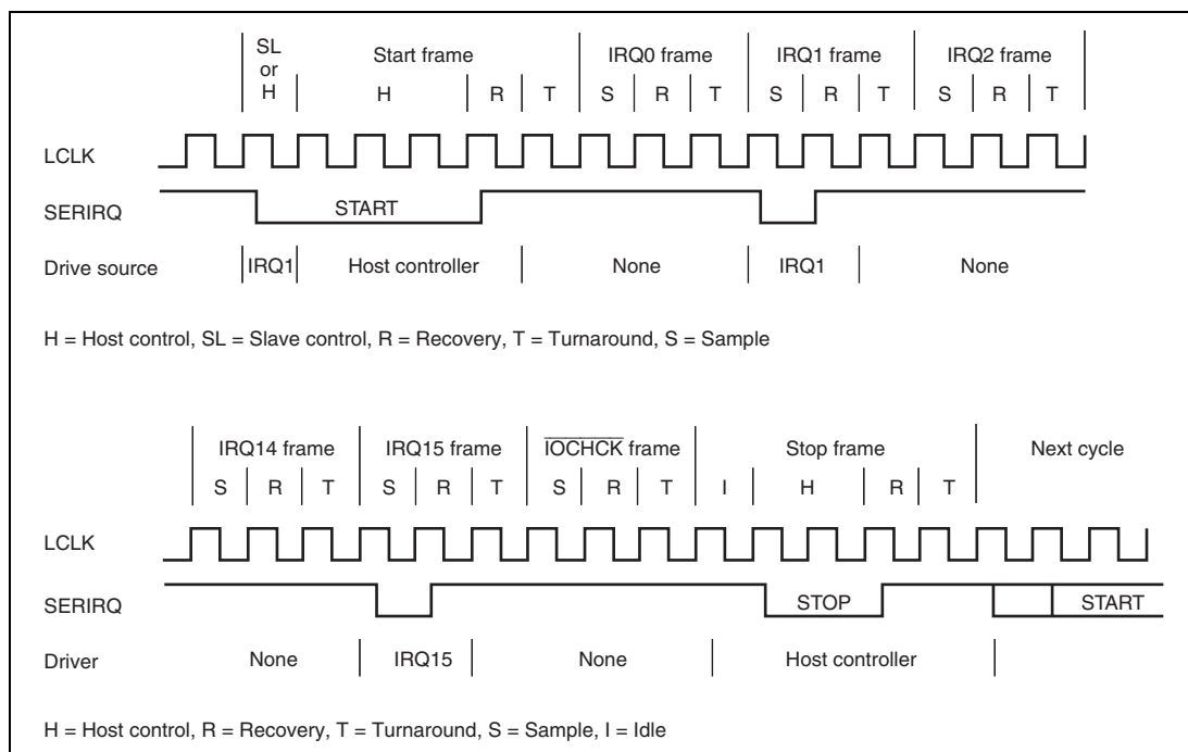
Figure 20.6 SERIRQ Timing
