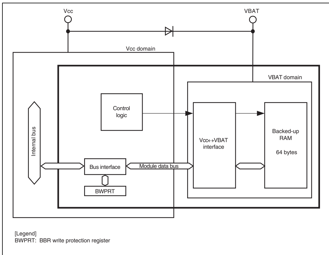
Figure 25.1 Block Diagram of BBR
