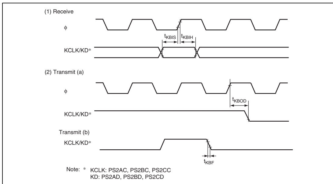
Figure 31.21 PS2 Timing
