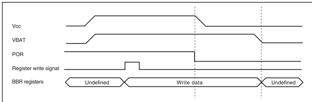
Figure 25.2 Retaining BBR Registers by VBAT Power
