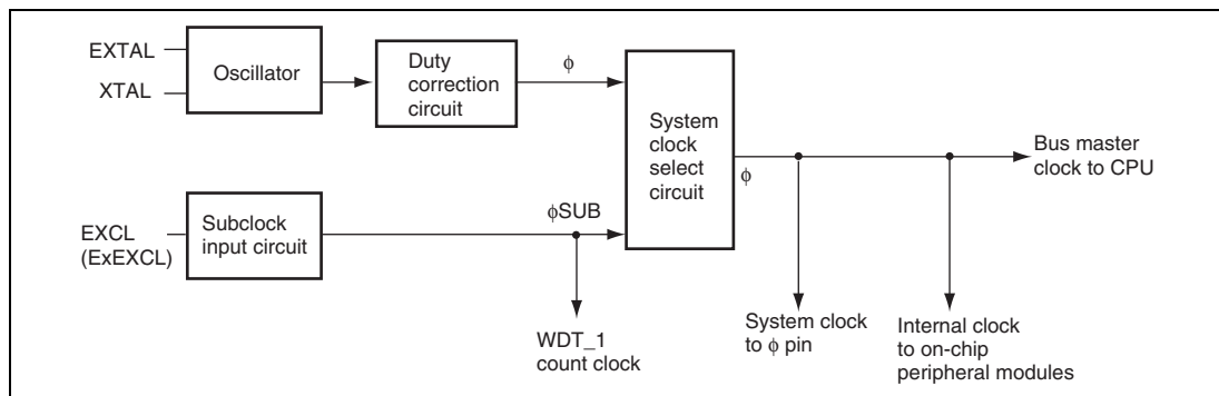
Figure 28.1 Block Diagram of Clock Pulse Generator
