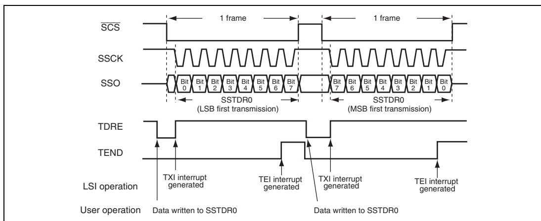
Figure 22.5 (1) Example of Transmission Operation (SSU Mode) When 8-bit data length is selected (SSTDR0 is valid) with CPOS = 0 and CPHS = 0
