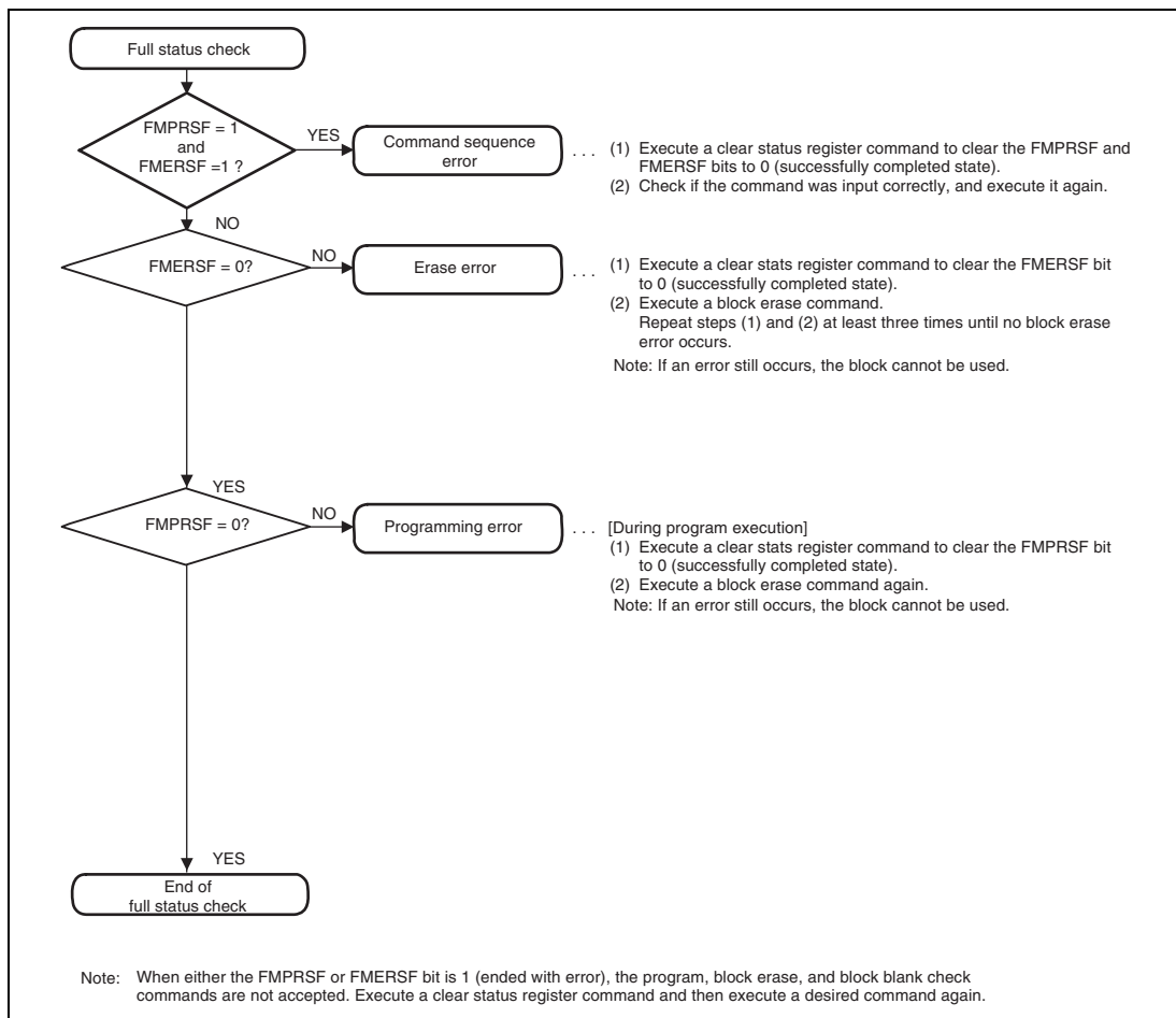
Figure 27.10 Flowchart of Full Status Check Processing and Corrective Actions for Each Error
