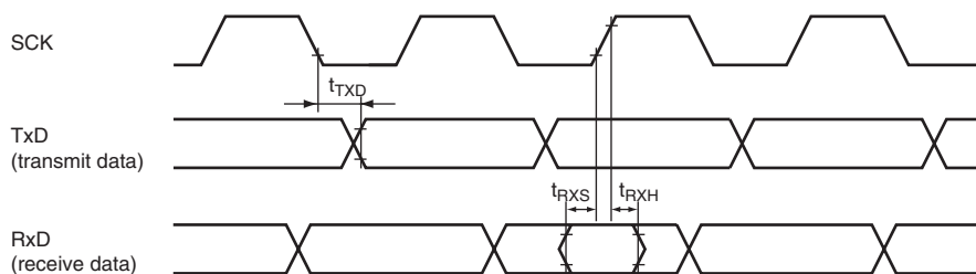
Figure 31.19 SCI Input/Output Timing (Clock Synchronous Mode)
