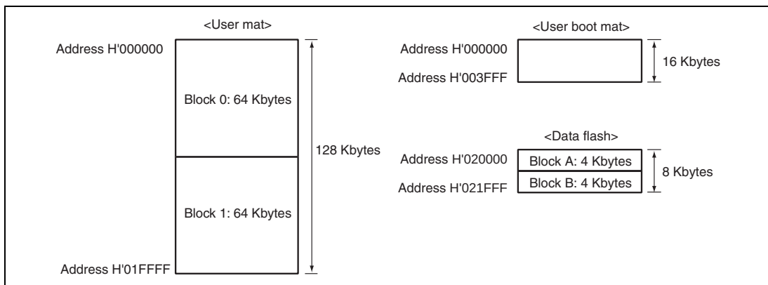
Figure 27.2 Flash Memory Configuration
