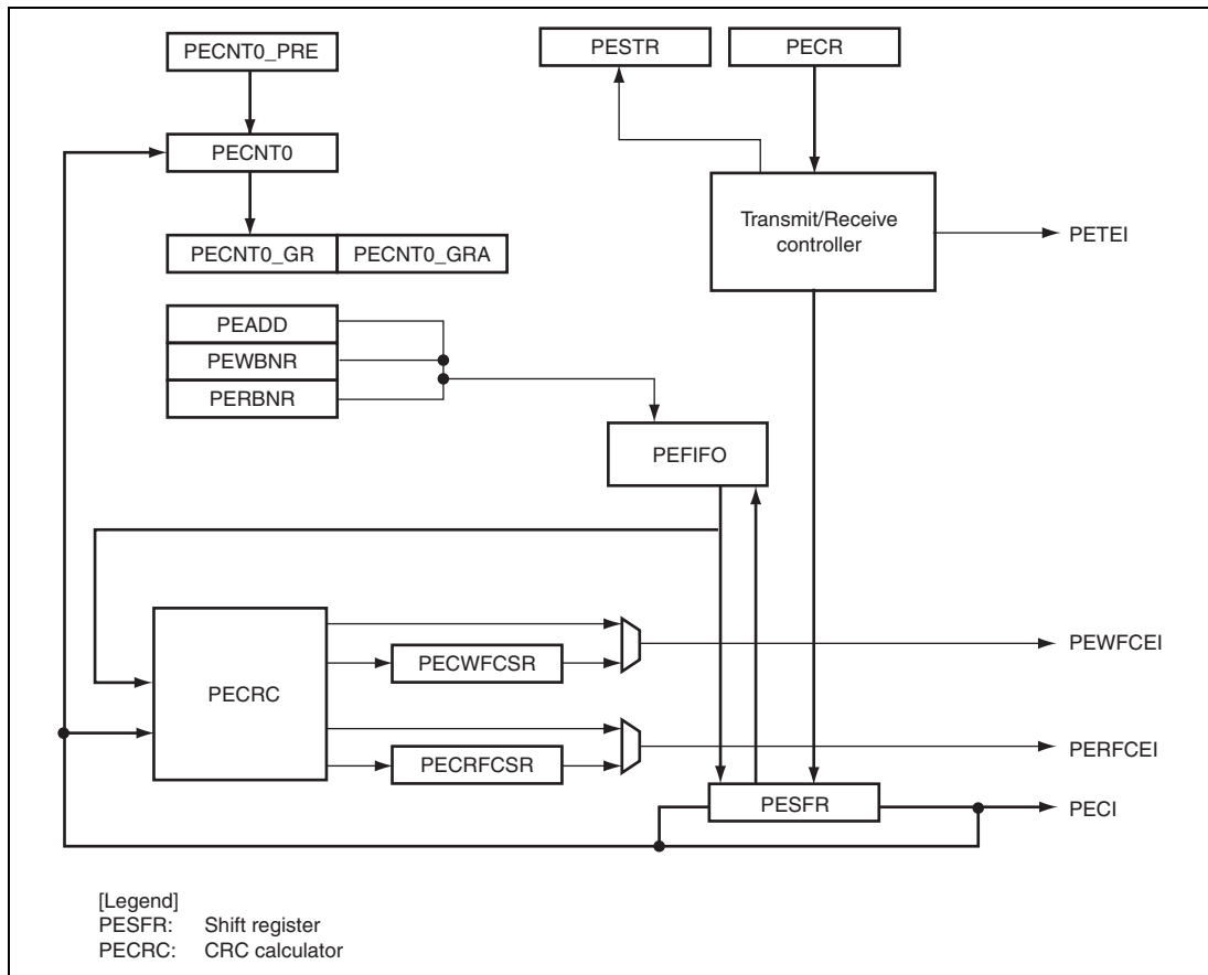
Figure 23.1 Block Diagram of PECI
