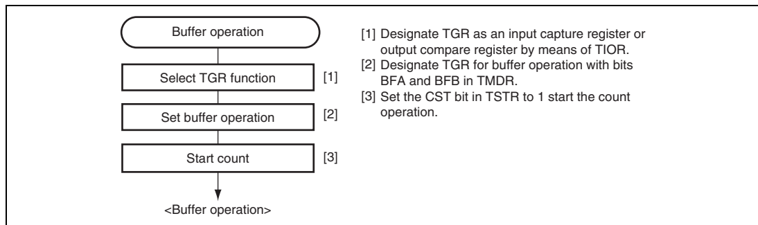
Figure 11.18 Example of Buffer Operation Setting Procedure
