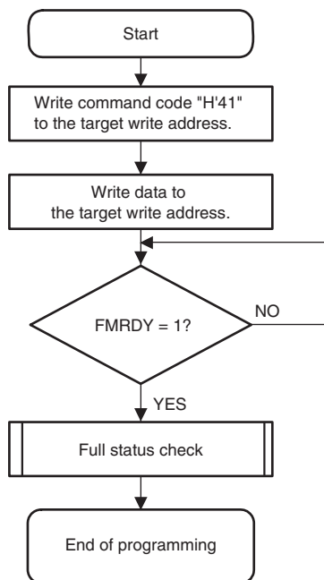
Figure 27.6 Flowchart of Program Command Processing
