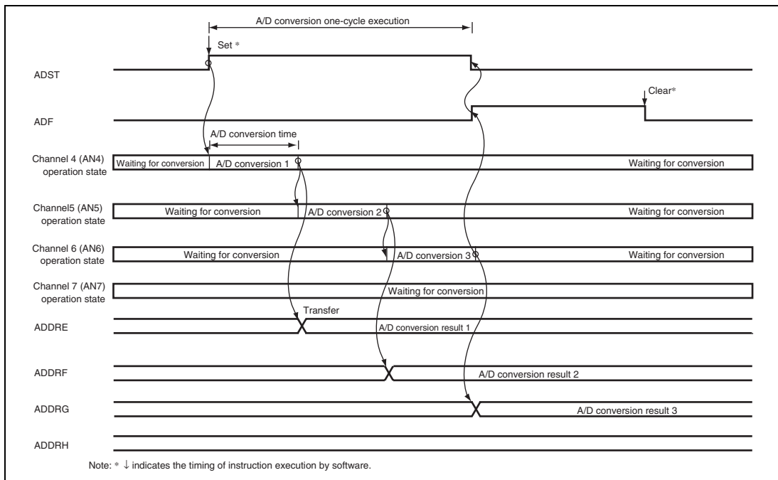
Figure 24.4 Example of A/D Conversion (One-Cycle Scan Mode, Three Channels (AN4 to AN6) Selected)
