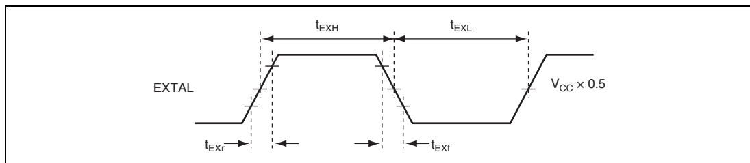
Figure 28.5 External Clock Input Timing
