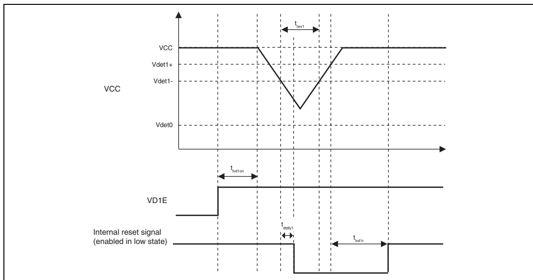
Figure 31.33 Electrical Characteristics of Low Voltage Detection Circuit 1
