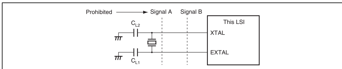
Figure 28.9 Note on Board Design of Oscillator Section
