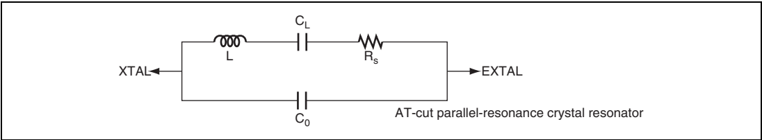
Figure 28.3 Equivalent Circuit of Crystal Resonator
