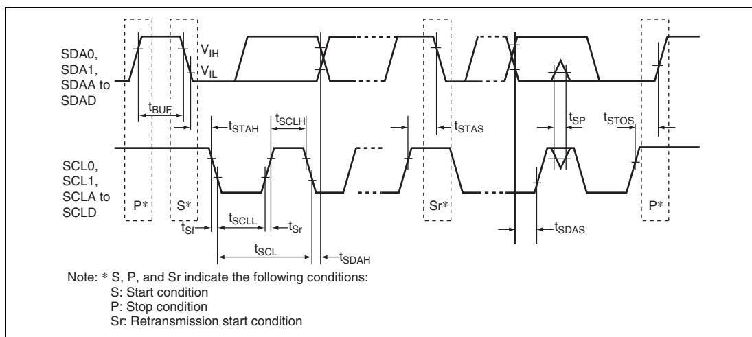
Figure 31.22 I 2 C Bus Interface Input/Output Timing
