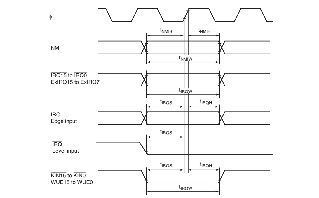
Figure 31.8 Interrupt Input Timing
