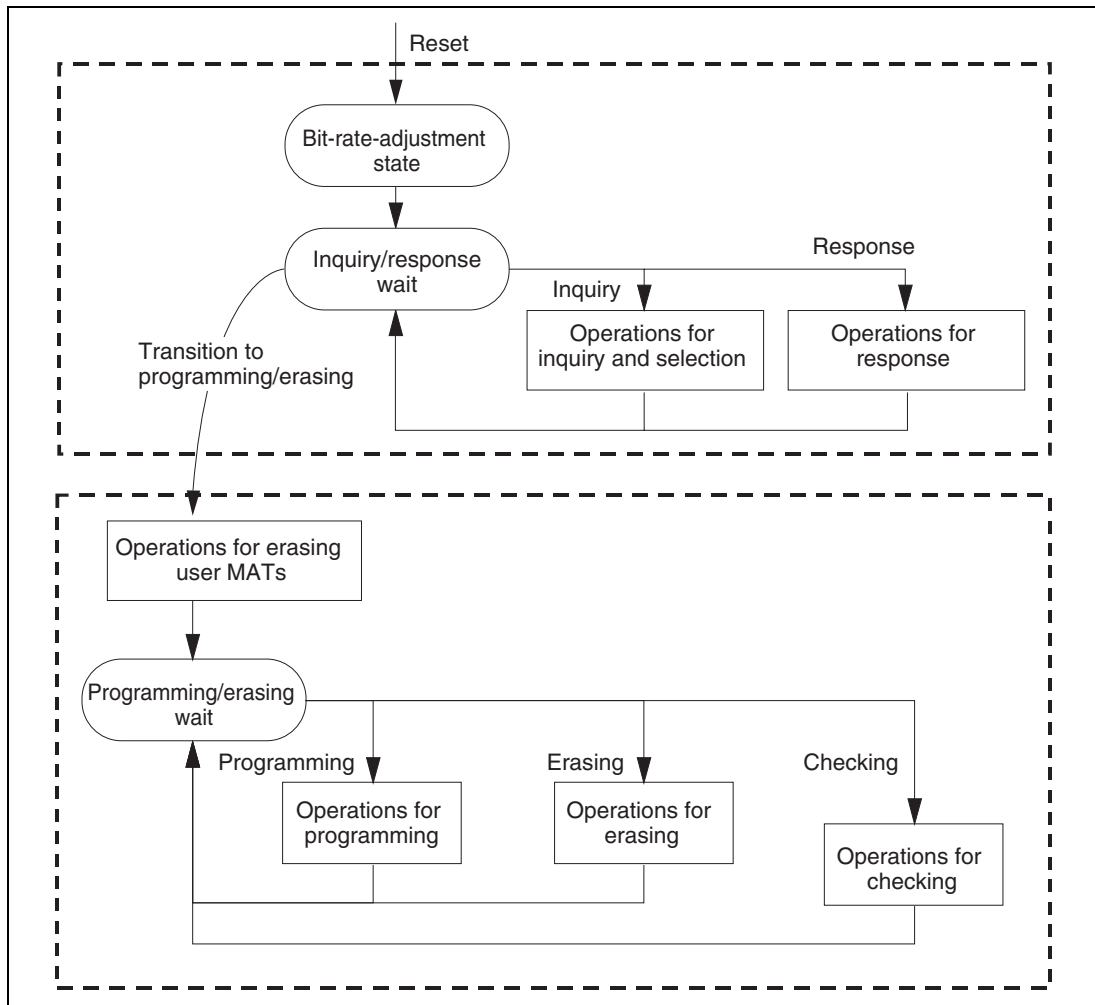
Figure 27.16 Boot Program States
