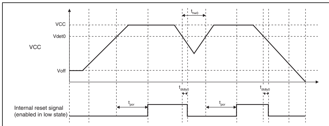
Figure 31.32 Electrical Characteristics of the Power-on Reset/Low Voltage Detection Circuit 0
