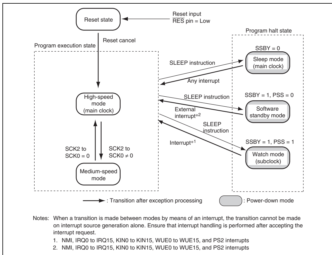
Figure 29.1 Mode Transition Diagram
