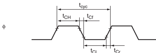
Figure 31.4 System Clock Timing
