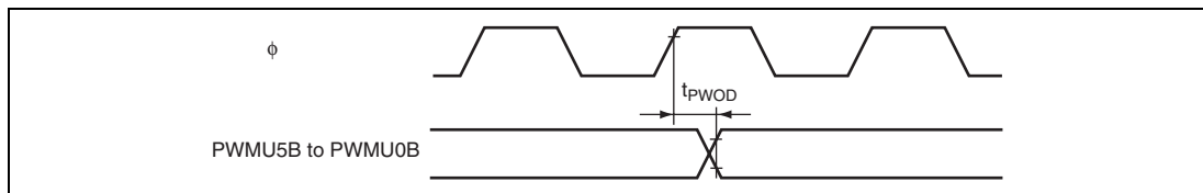
Figure 31.17 PWMU Output Timing
