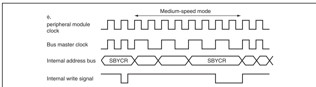
Figure 29.2 Timing of Medium-Speed Mode
