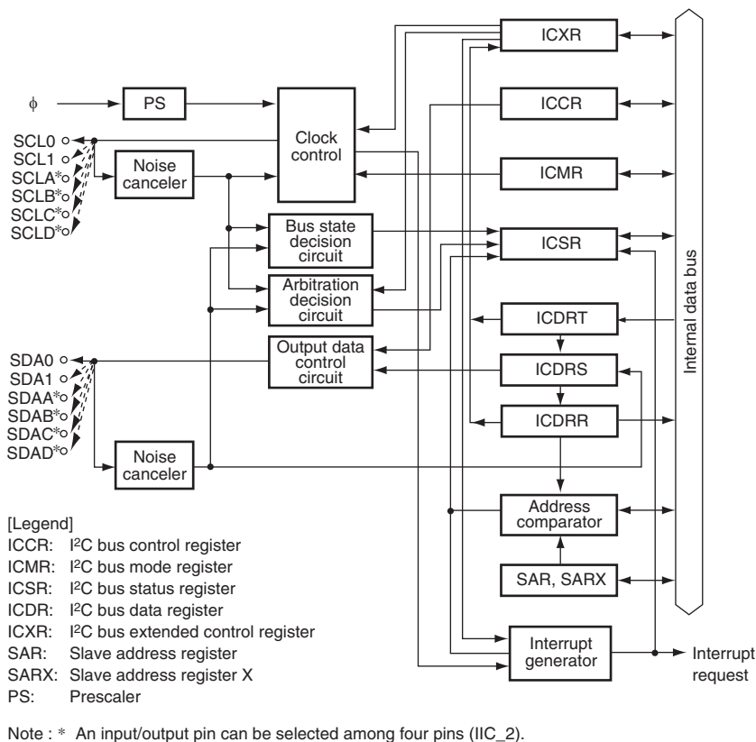
Figure 17.1 Block Diagram of I 2 C Bus Interface
