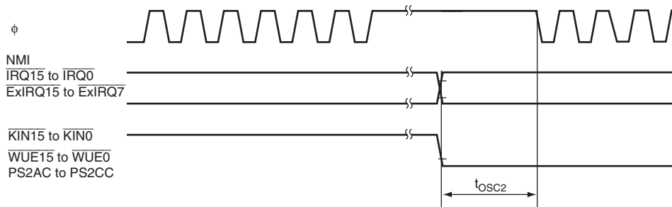
Figure 31.6 Oscillation Stabilization Timing (Returning from Software Standby Mode)
