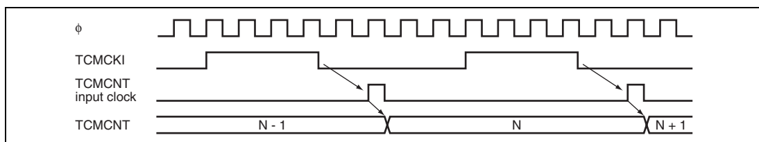
Figure 13.3 Count Timing of External Clock Operation (Falling Edges)
