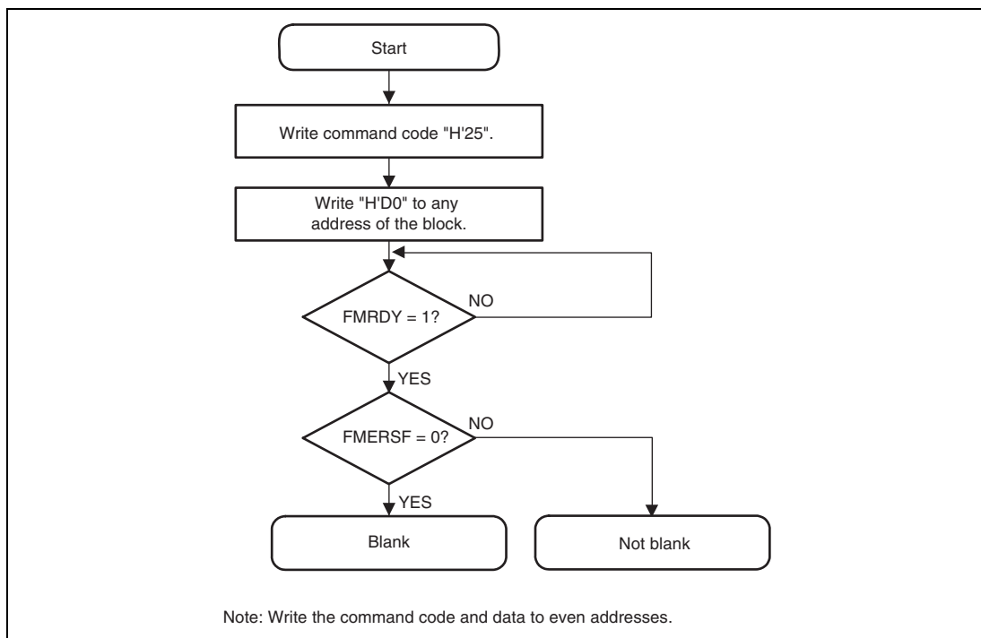
Figure 27.8 Flowchart of Block Blank Check Command Processing
