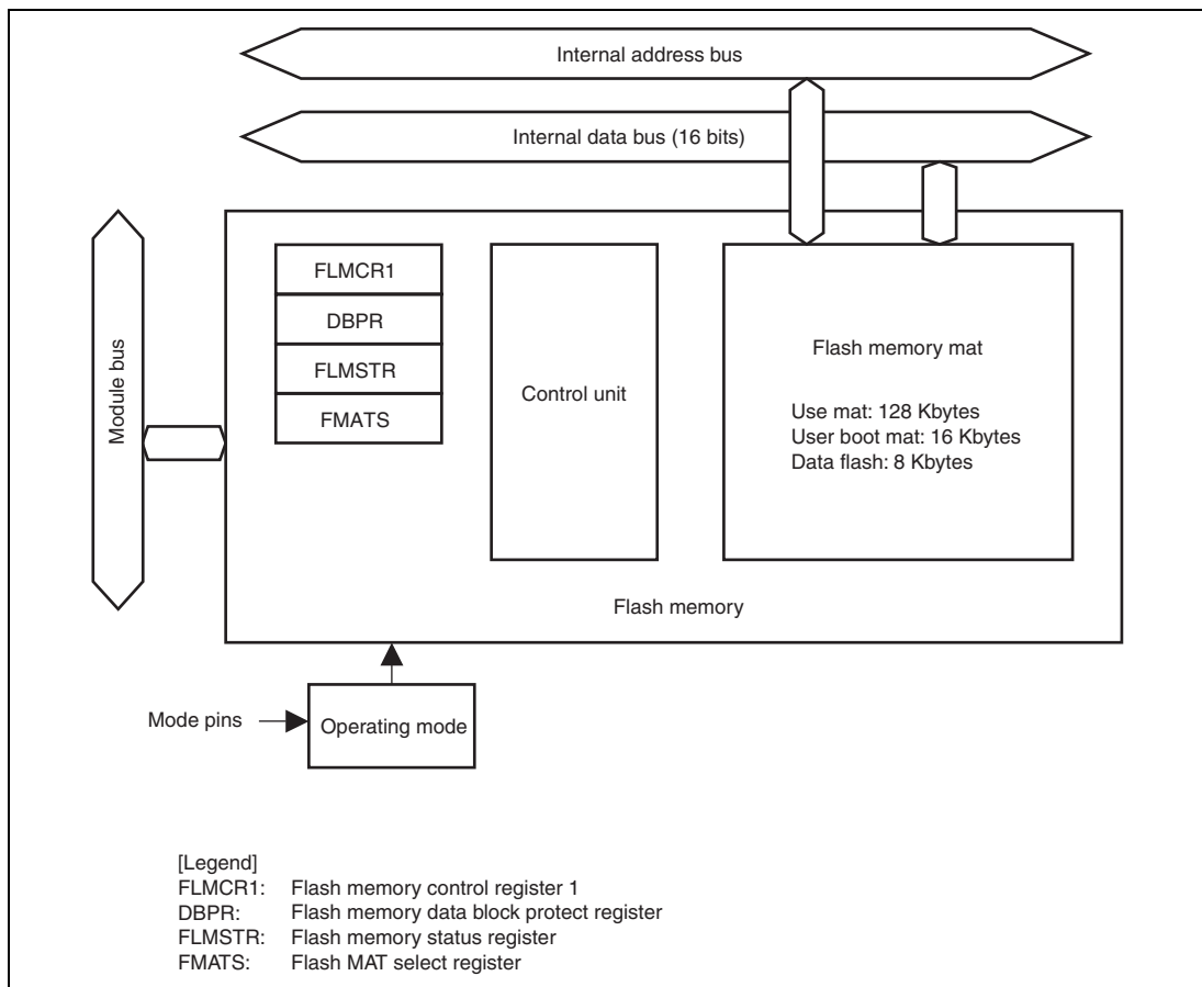
Figure 27.1 Block Diagram of Flash Memory
