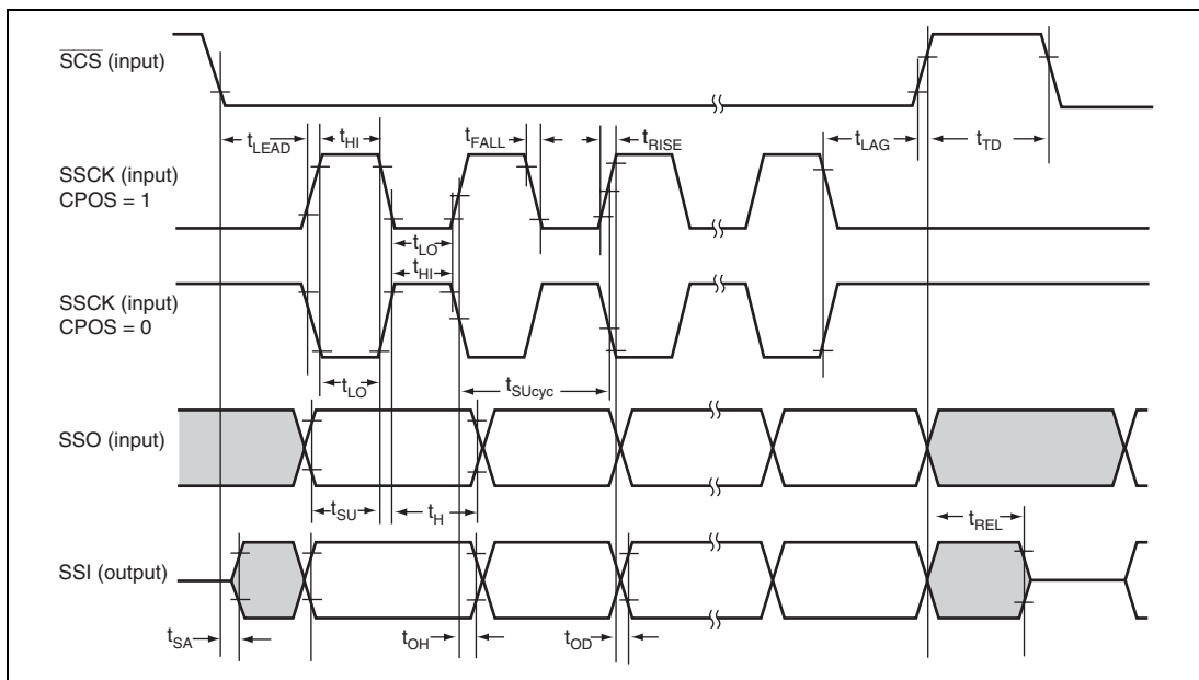
Figure 31.31 SSU Timing (Slave, CPHS = 0)
