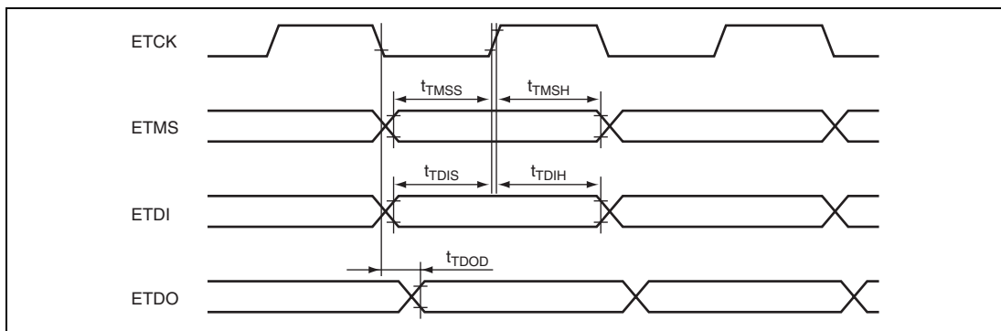
Figure 31.27 JTAG Input/Output Timing
