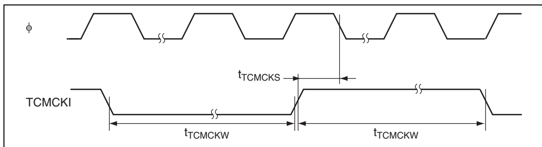
Figure 31.16 TCM Clock Input Timing
