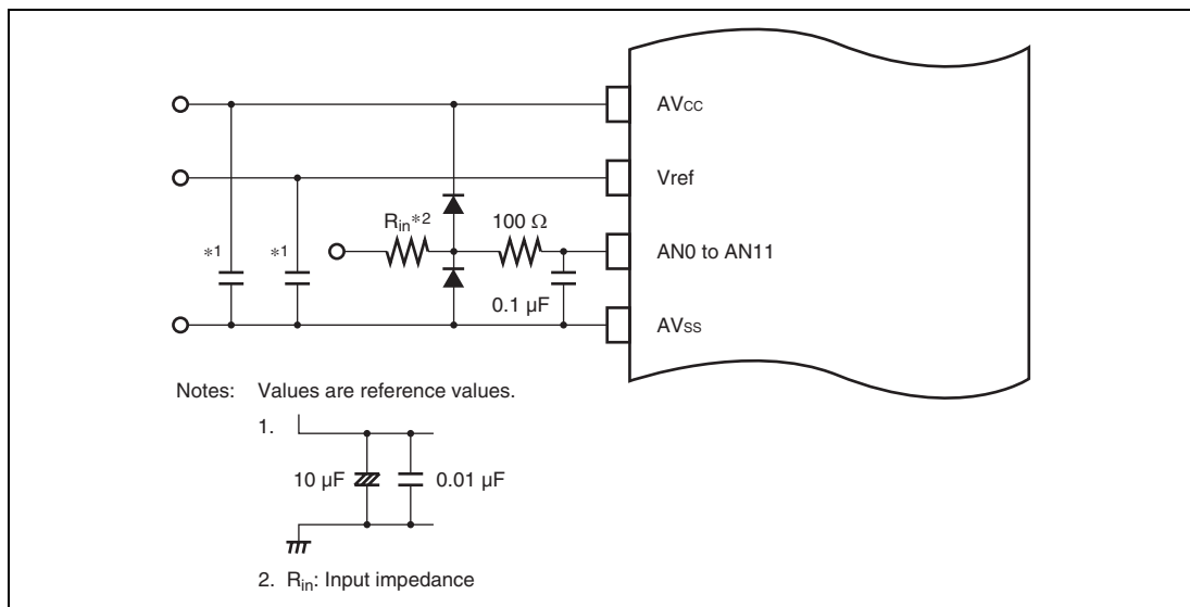
Figure 24.9 Example of Analog Input Protection Circuit
