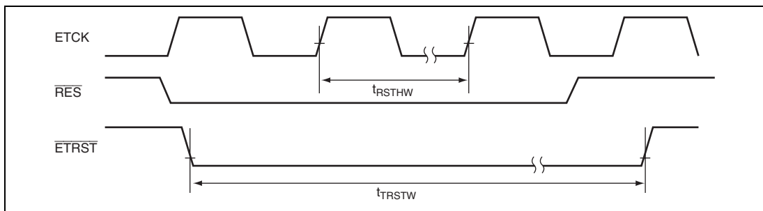
Figure 31.26 Reset Hold Timing
