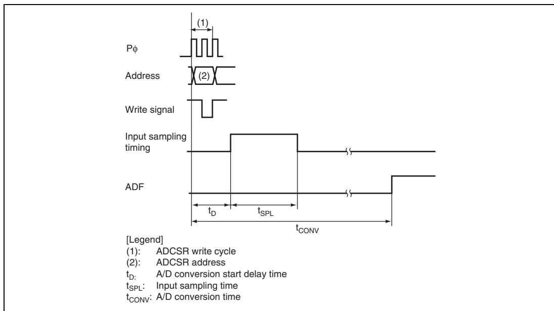
Figure 24.5 A/D Conversion Timing
