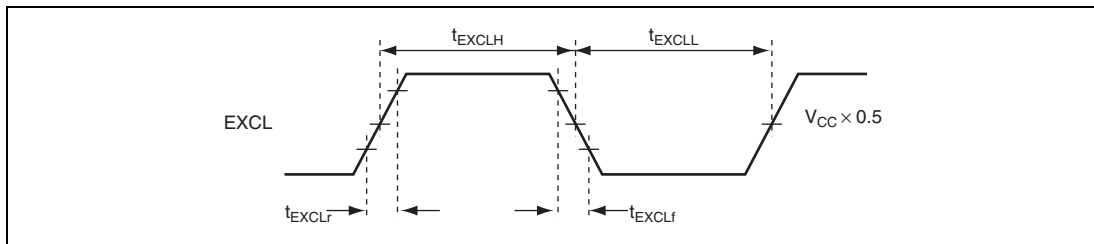
Figure 28.8 Subclock Input Timing
