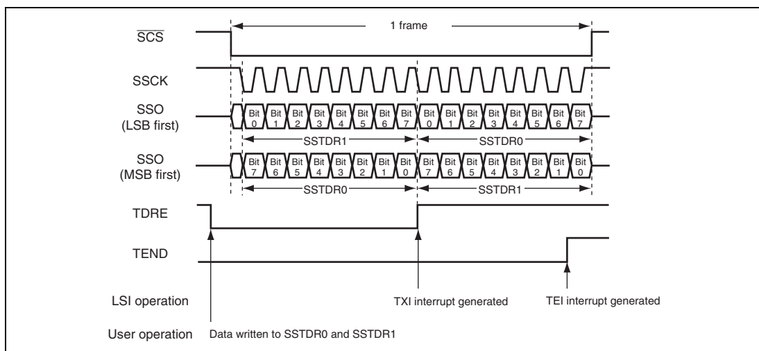
Figure 22.5 (2) Example of Transmission Operation (SSU Mode) When 16-bit data length is selected (SSTDR0 and SSTDR1 are valid) with CPOS = 0 and CPHS = 0
