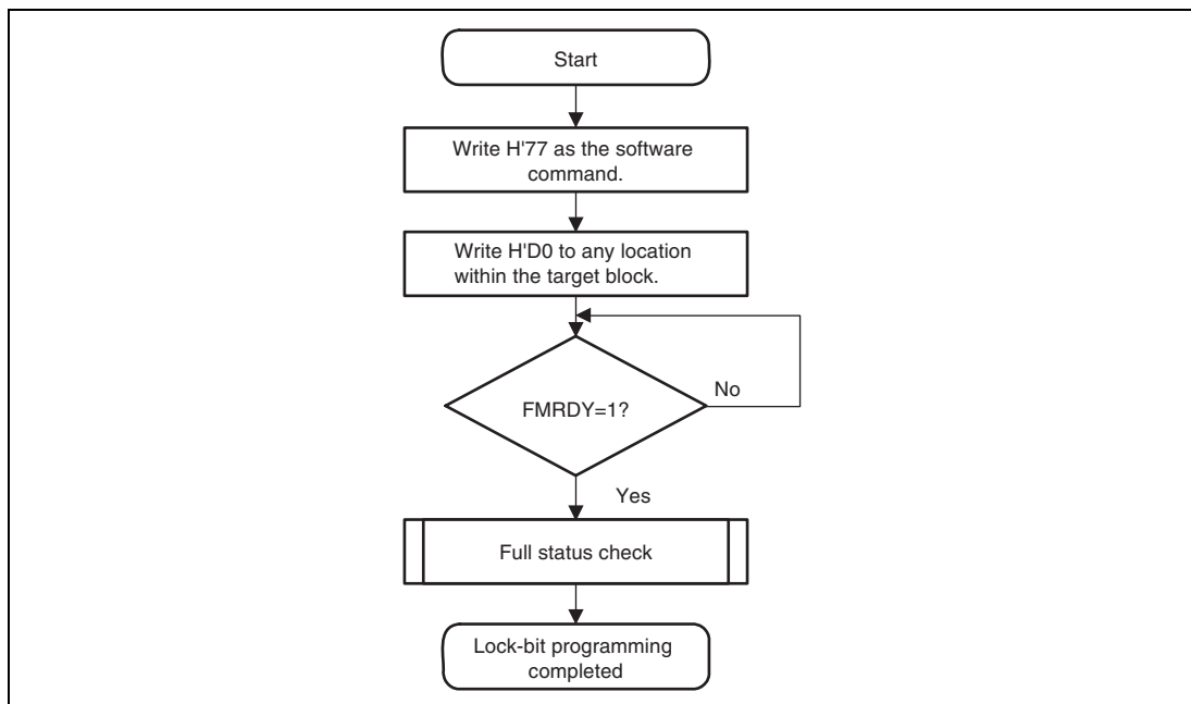
Figure 27.9 Flowchart of Lock-Bit Programming
