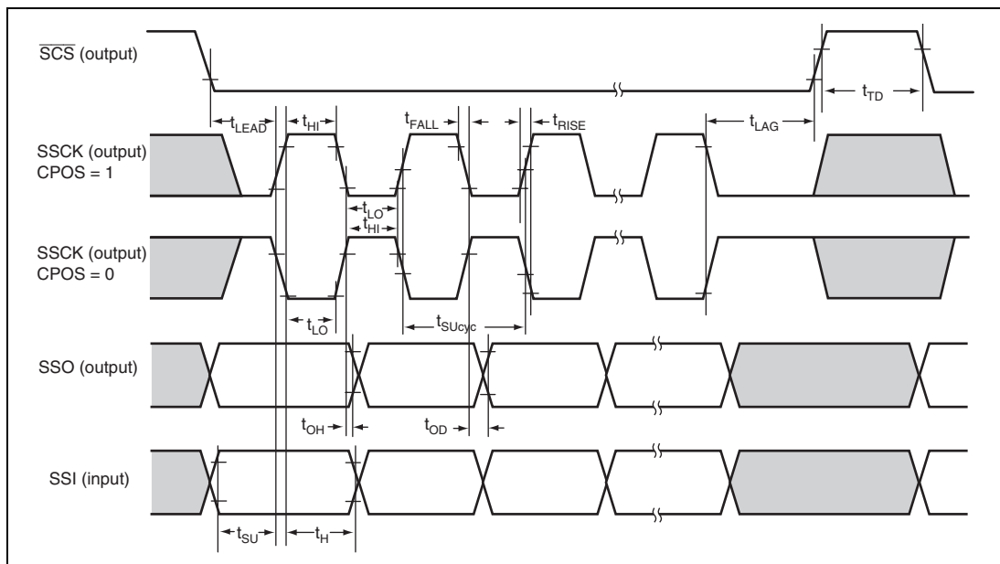
Figure 31.28 SSU Timing (Master, CPHS = 1)
