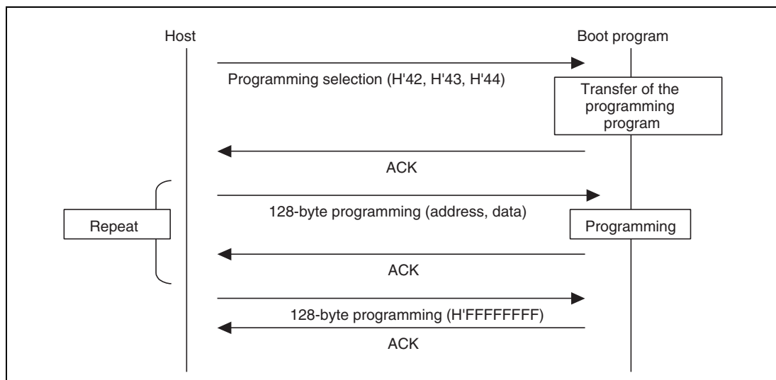
Figure 27.20 Programming Sequence
