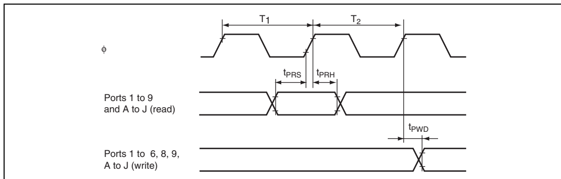
Figure 31.9 I/O Port Input/Output Timing
