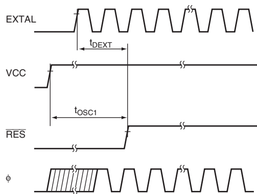
Figure 31.5 Oscillation Stabilization Timing
