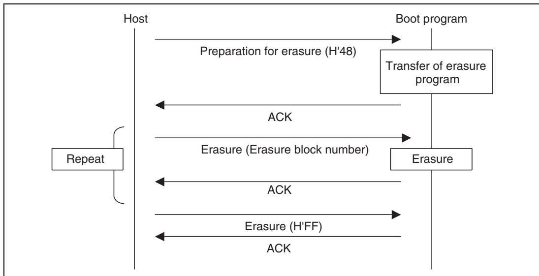
Figure 27.21 Erasure Sequence
