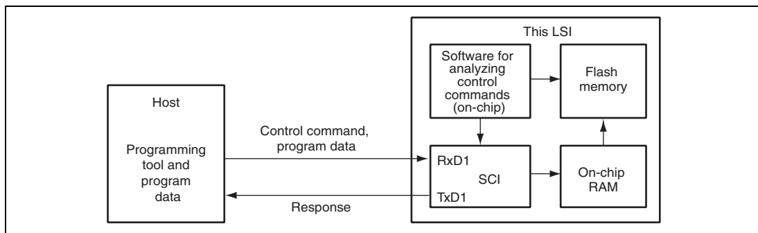
Figure 27.11 System Configuration in Boot Mode
