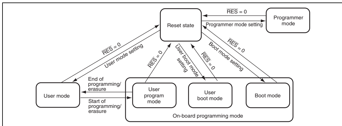
Figure 27.4 Mode Transition of Flash Memory
