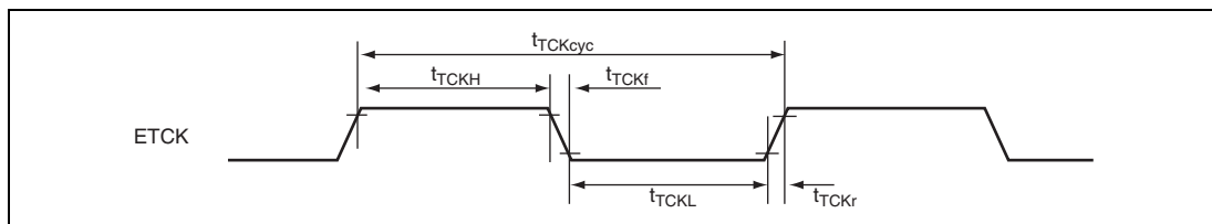
Figure 31.25 JTAG ETCK Timing
