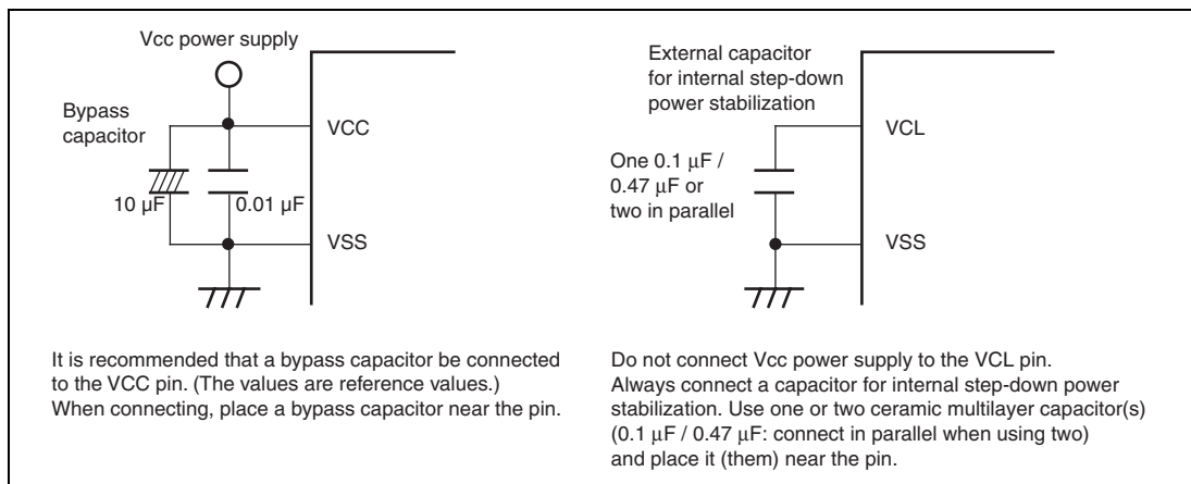
Figure 31.34 Connection of VCL Capacitor
