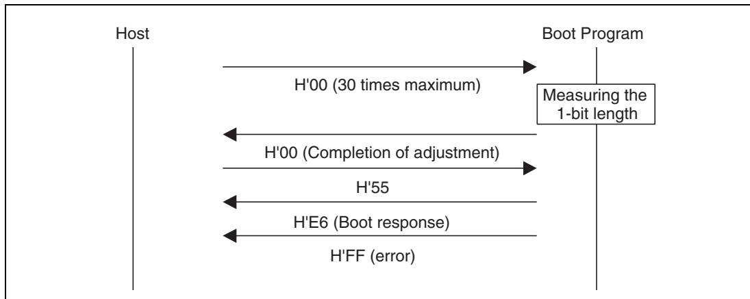
Figure 27.17 Bit-Rate-Adjustment Sequence
