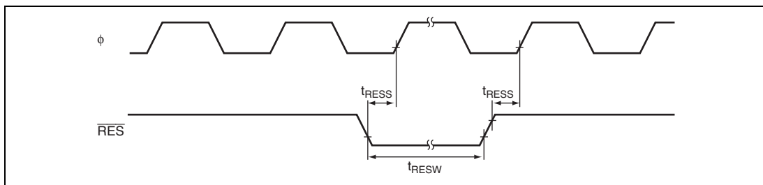
Figure 31.7 Reset Input Timing
