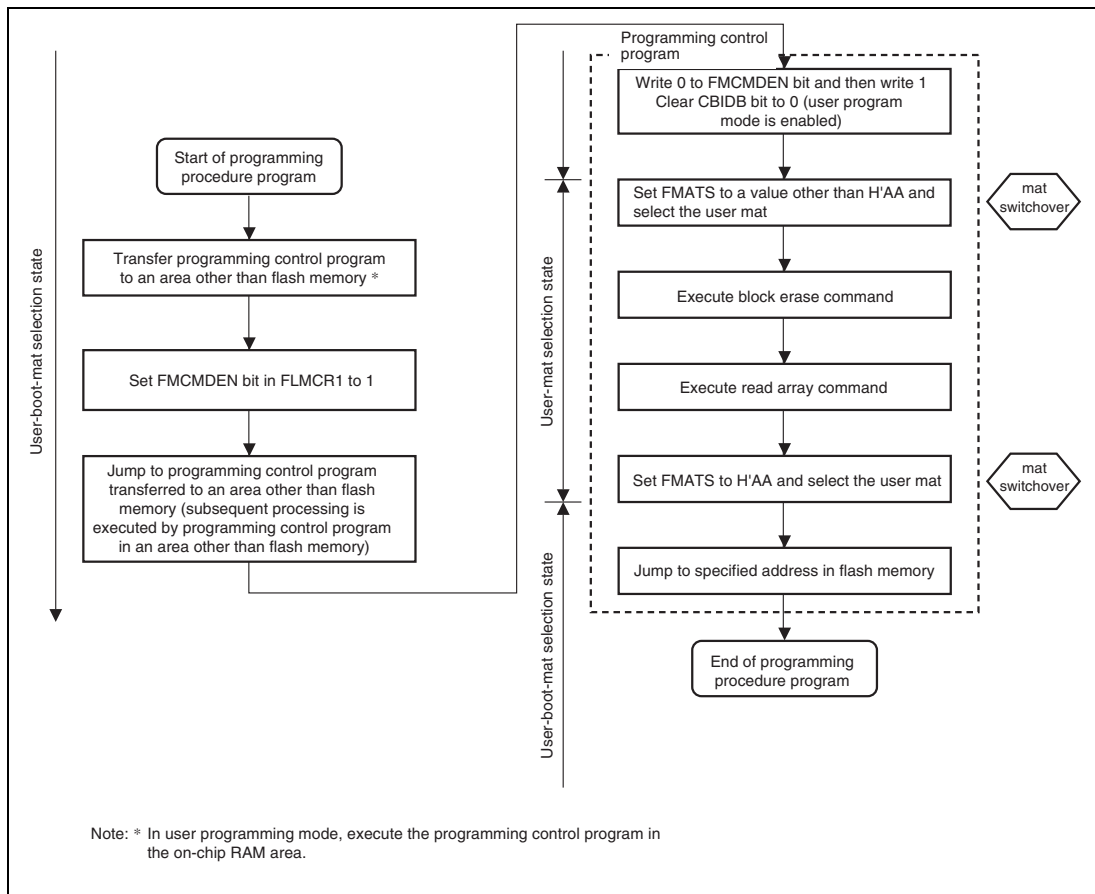
Figure 27.14 Procedure for Erasing User Mat in User Boot Mode
