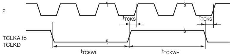
Figure 31.11 TPU Clock Input Timing
