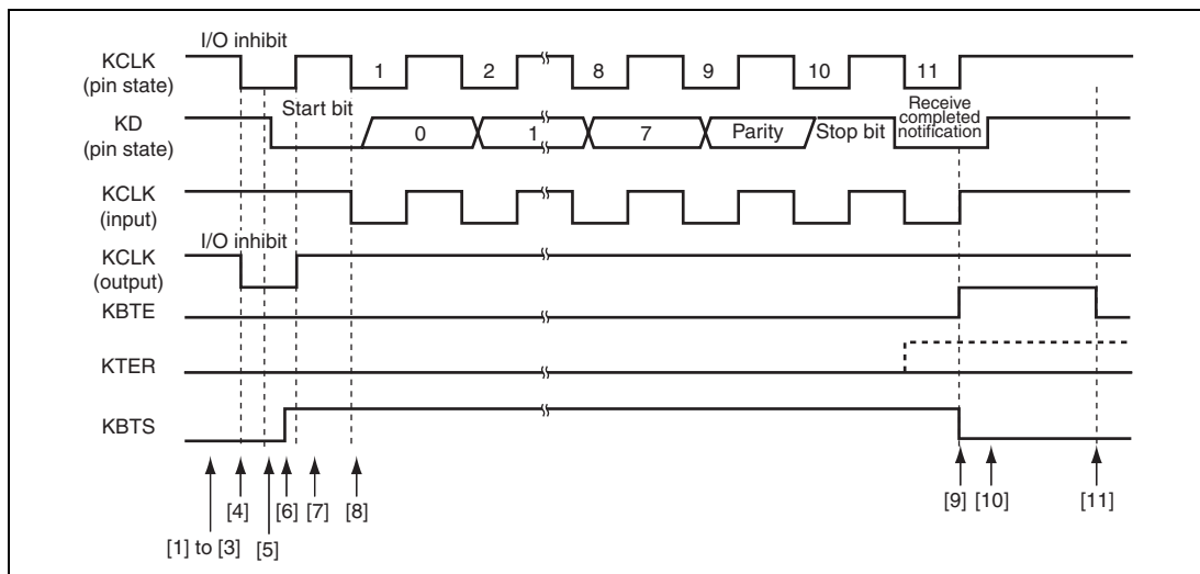
Figure 19.6 Transmit Timing
