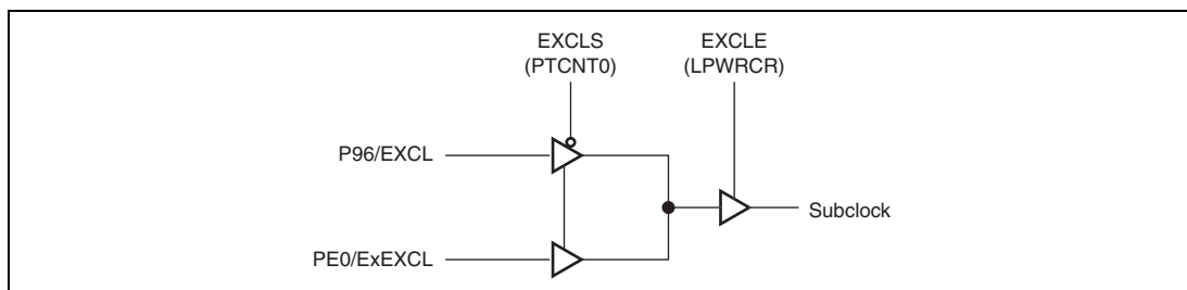
Figure 28.7 Subclock Input from EXCL Pin and ExEXCL Pin
