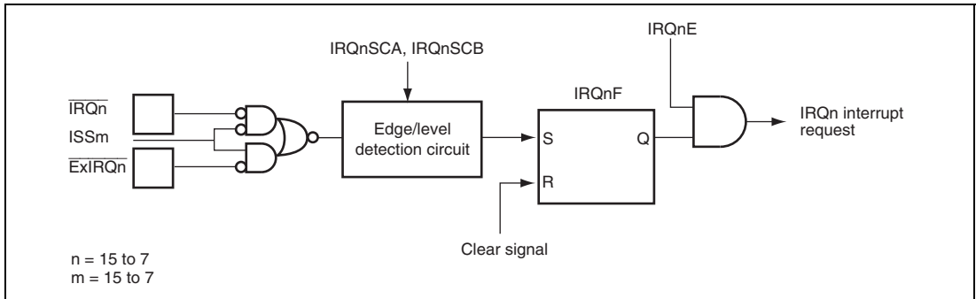
Figure 7.3 Block Diagram of Interrupts IRQ15 to IRQ0
