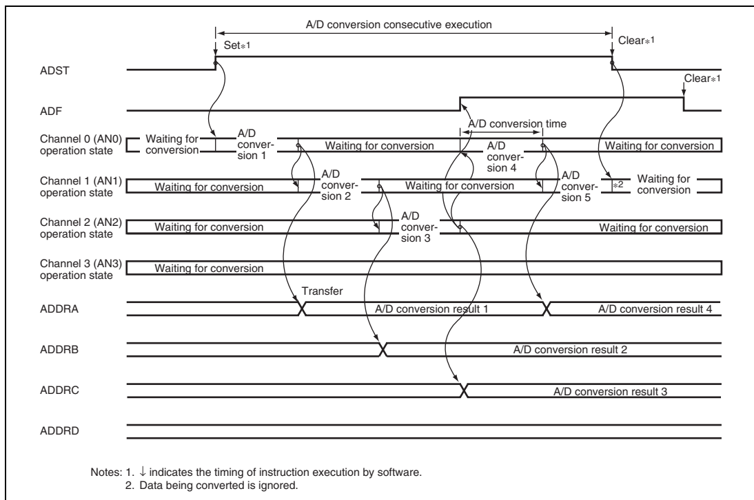
Figure 24.3 Example of A/D Conversion (Continuous Scan Mode, Three Channels (AN0 to AN2) Selected)
