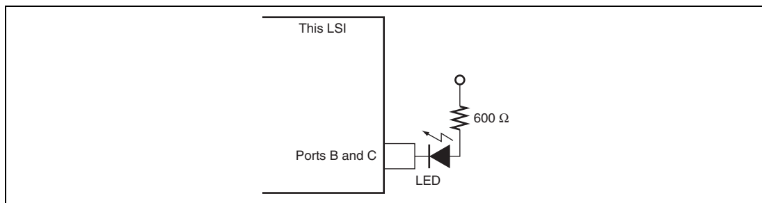
Figure 31.2 LED Drive Circuit (Example)
