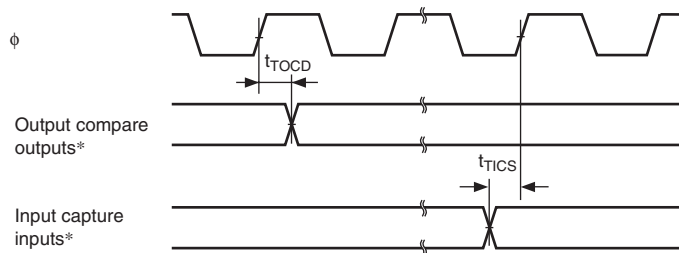
Figure 31.10 TPU Input/Output Timing
