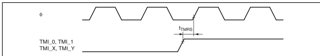
Figure 31.14 8-Bit Timer Reset Input Timing
