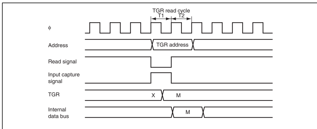
Figure 11.48 Conflict between TGR Read and Input Capture
