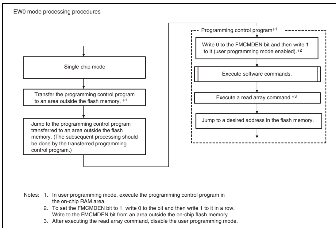
Figure 27.5 Setting and Clearing EW0 Mode
