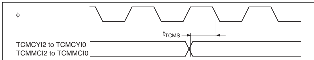
Figure 31.15 TCM Input Setup Time
