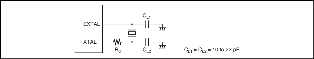
Figure 28.2 Typical Connection to Crystal Resonator
