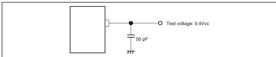
Figure 31.24 Test Conditions for Tester
