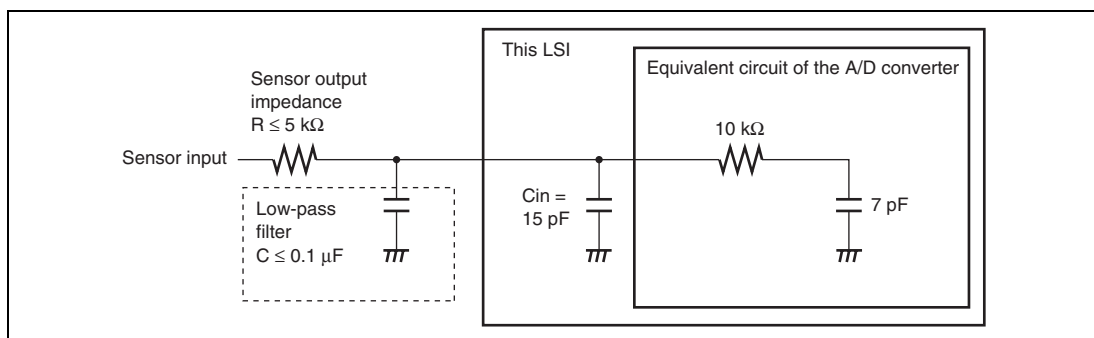
Figure 24.8 Example of Analog Input Circuit
