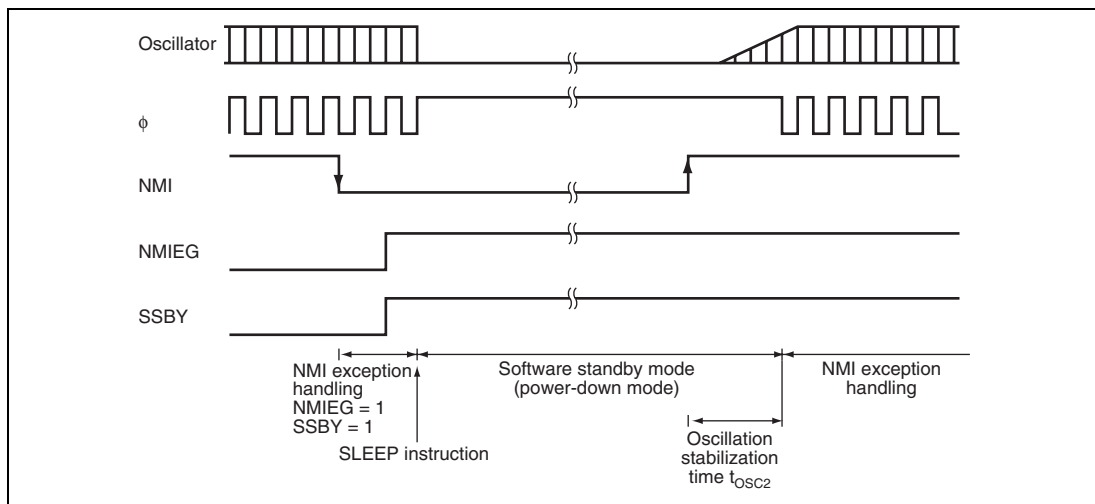
Figure 29.3 Software Standby Mode Application Example
