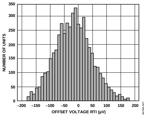
Figure 7. Typical Distribution of Offset Voltage, V_{OSI}
