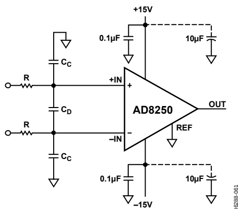
Figure 54. RFI Suppression
