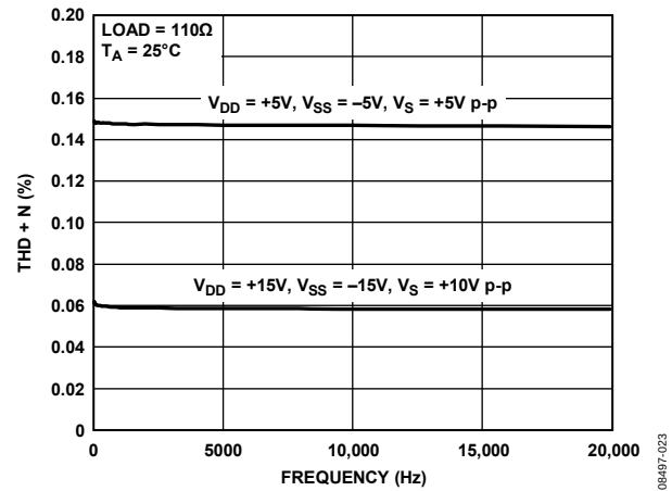
Figure 21. THD + N vs. Frequency, \pm 15\text{ V} Dual Supply
