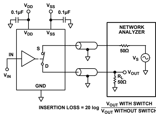
Figure 28. Insertion Loss
