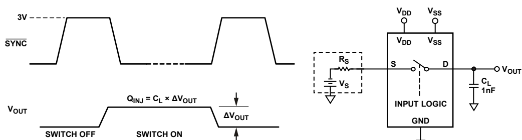
Figure 31. Charge Injection
