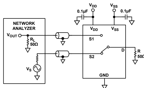
Figure 27. Channel-to-Channel Crosstalk
