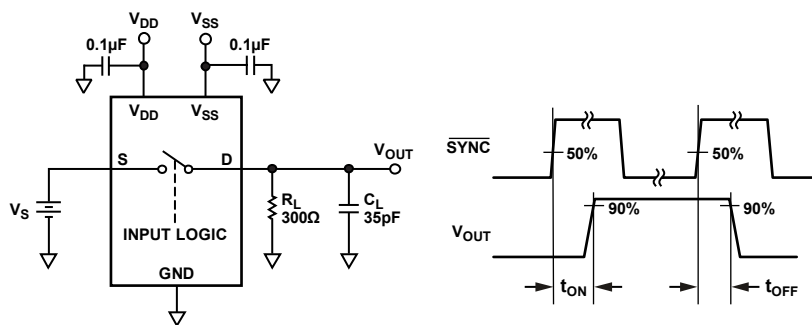
Figure 30. Switching Times
