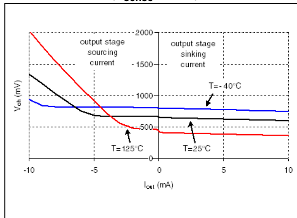
Figure 8. Output stage high-state saturation voltage versus output current ( V_{\text{sense}} = +1\text{ V} )
