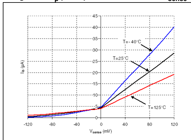
Figure 4. V_{\text{p}} pin input bias current vs. V_{\text{sense}}
