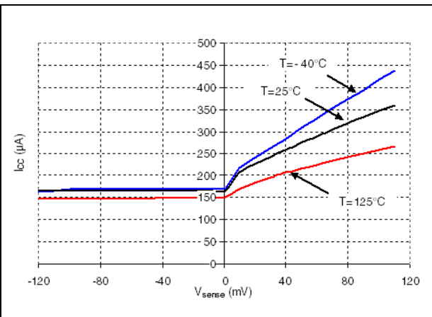
Figure 5. V_{\text{m}} pin input bias current vs. V_{\text{sense}}
