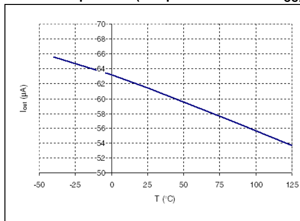
Figure 10. Output short-circuit sink current versus temperature (Out pin connected to V_{\text{CC}} )
