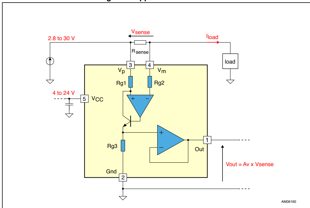
Figure 1. Application schematic
