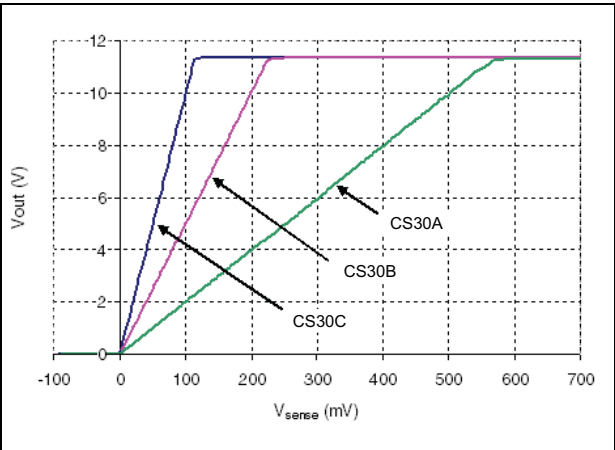
Figure 17. Output voltage versus V_{\text{sense}}
