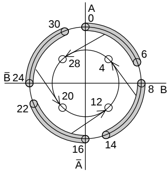
1-2 phase → 2 phase
