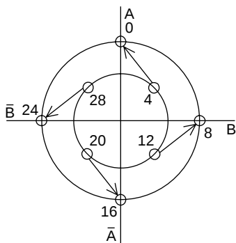
2 phase → 1-2 phase
