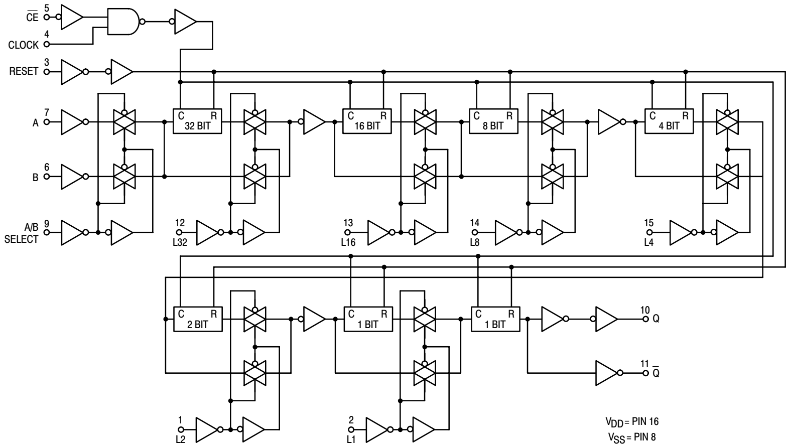
Figure 1. Logic Diagram
