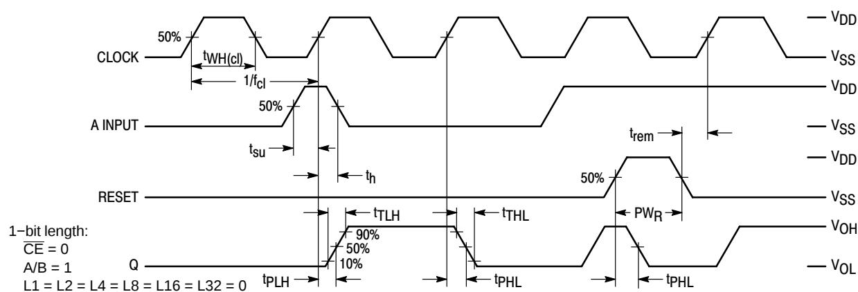
Figure 4. Timing Diagram
