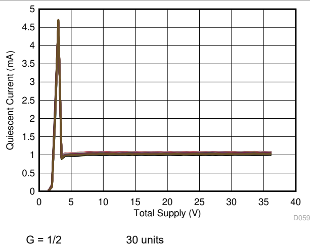
Figure 7-59. Supply Current vs Supply Voltage
