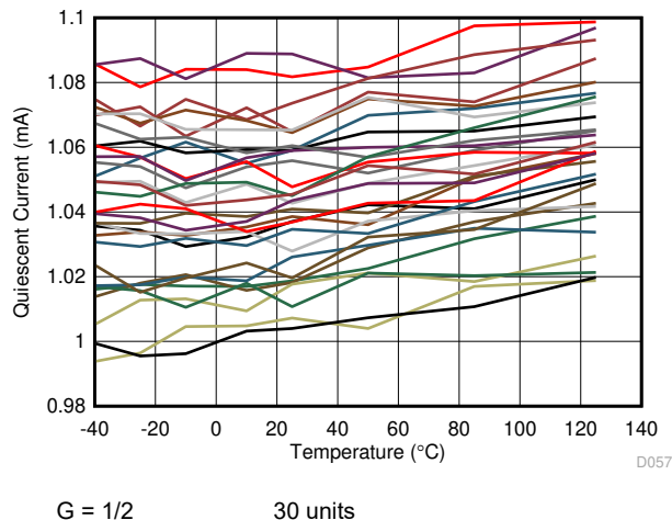
Figure 7-57. Supply Current vs Temperature
