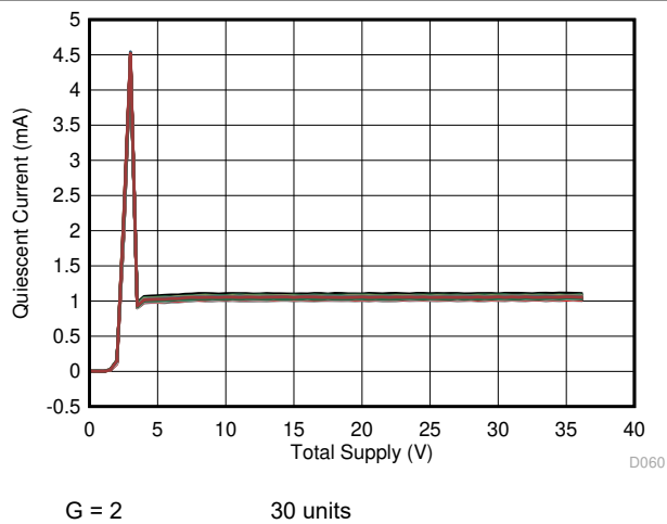
Figure 7-60. Supply Current vs Supply Voltage
