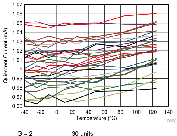
Figure 7-58. Supply Current vs Temperature
