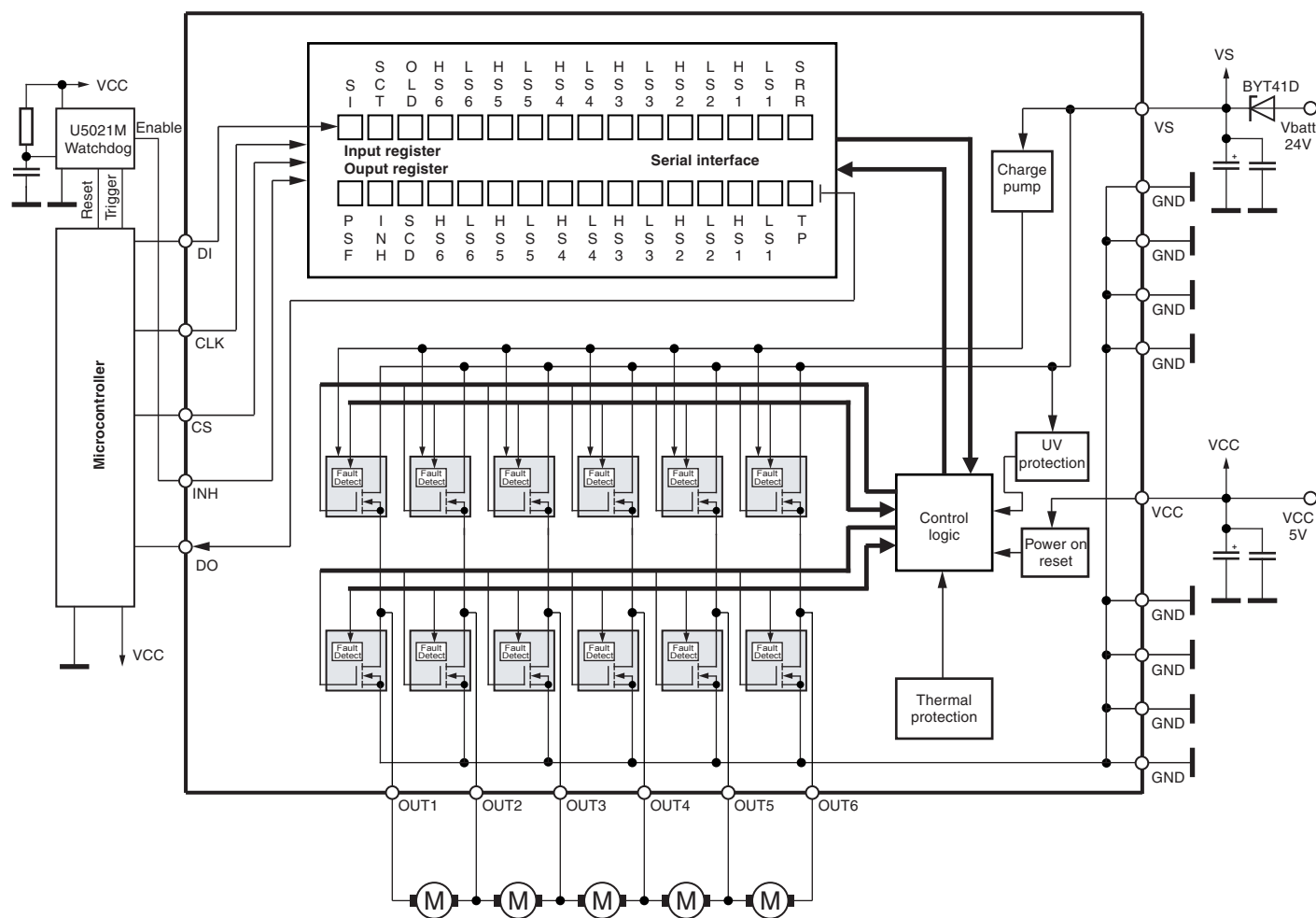
Figure 10-1. Application Circuit
