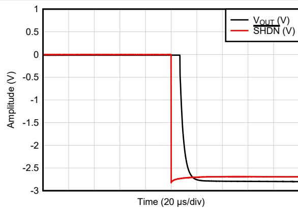
Figure 7-44. Amplifier Disable Response
