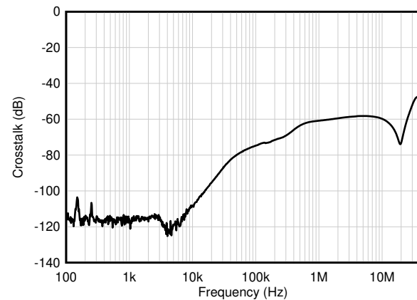
Figure 7-46. Channel Separation
