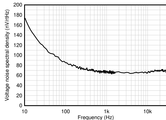
Figure 7-22. Input Voltage Noise Spectral Density
