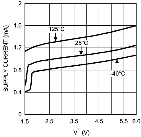
Supply Current vs. Supply Voltage (LMV796/LMV796Q)
