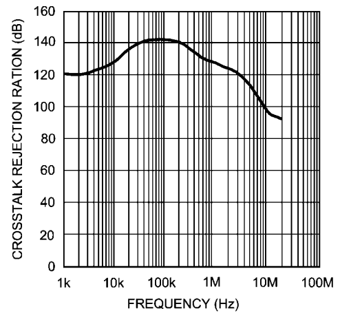
Crosstalk Rejection
