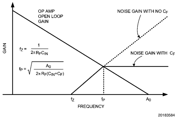
FIGURE 9. C_F Selection for Stability
