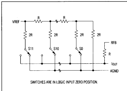
Figure 1. MX7549 Simplified DAC Schematic
