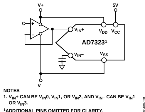
Figure 39. Pseudo Differential Inputs
