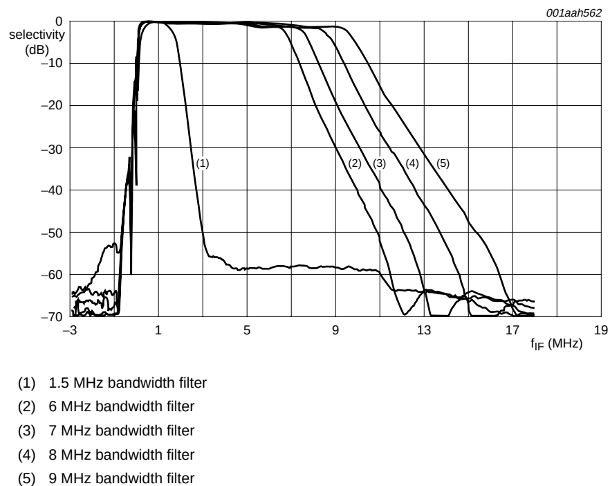
Fig 24. Typical IF selectivity curves
