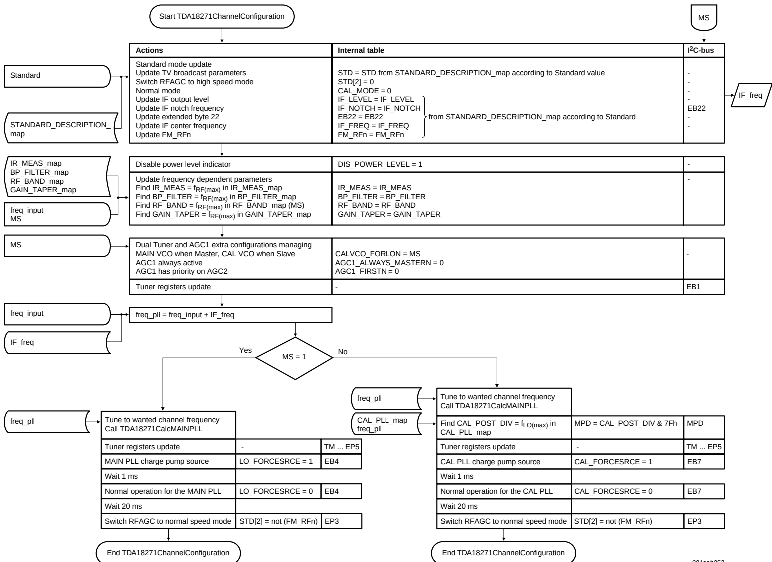
Fig 17. Flowchart TDA18271ChannelConfiguration
