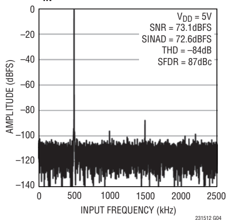
16k Point FFT, f_S = 5\text{Mps} f_{\text{IN}} = 500\text{kHz}
