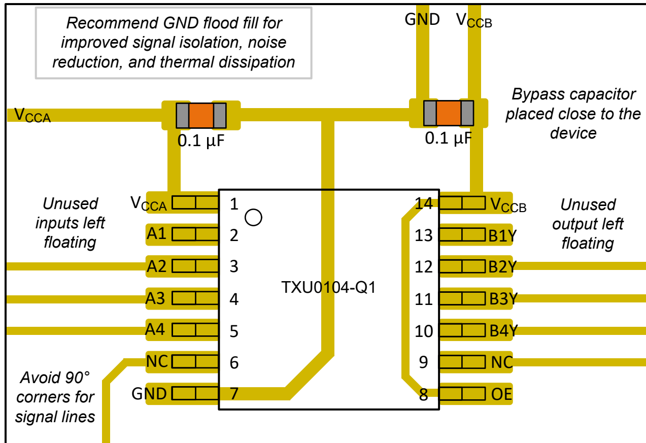
Figure 12-1. Layout Example – TXU0104-Q1
