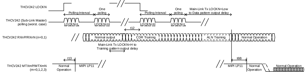
Figure 16. Re-Lock Sequence
