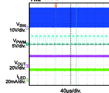
PWM Input Analog Dimming f_{PWM}=50kHz
