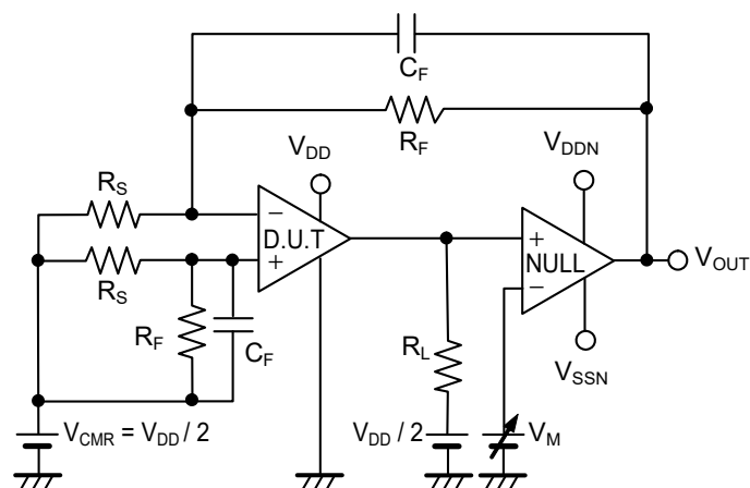
Figure 12 Test Circuit 8
