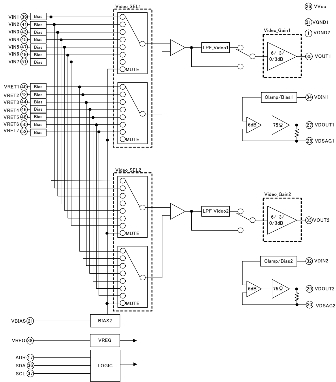
Fig.2 Block Diagram
