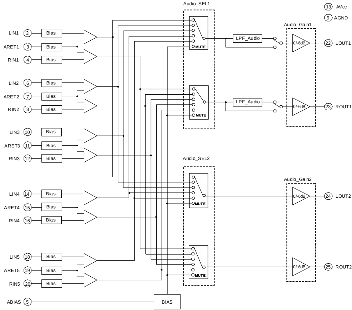
Fig.1 Block Diagram
