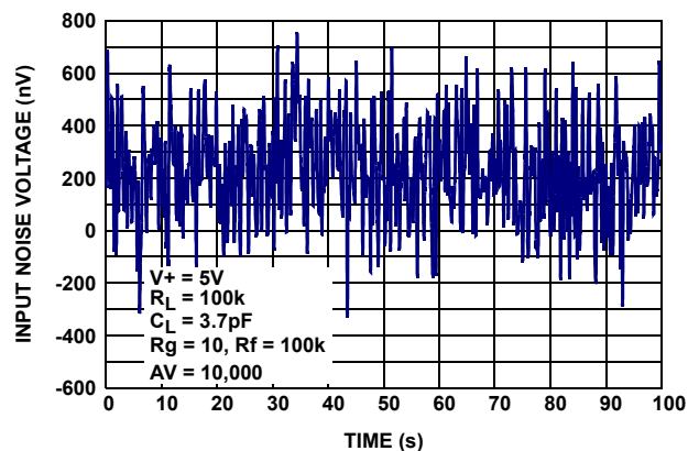
FIGURE 12. INPUT NOISE VOLTAGE 0.01Hz TO 10Hz
