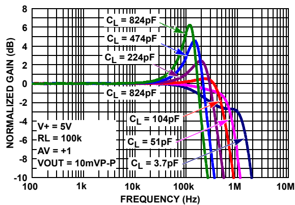
FIGURE 47. CHARACTERIZED GAIN vs FREQUENCY vs C_L
