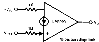
Comparator
