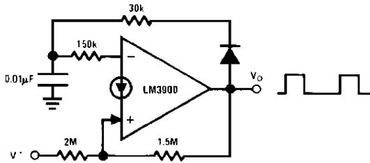
Pulse Generator
