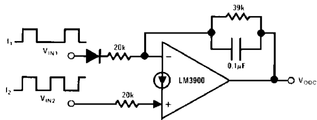
Frequency Differencing Tachometer
