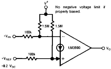
Low-Voltage Comparator
