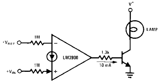
Power Comparator
