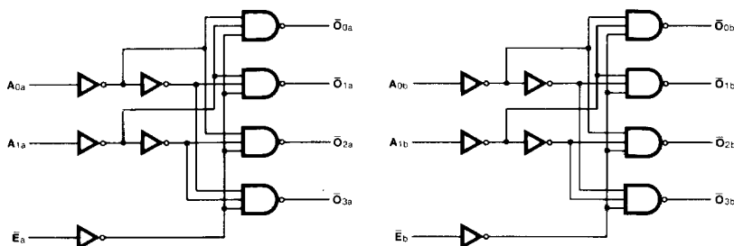
LOGIC DIAGRAM
