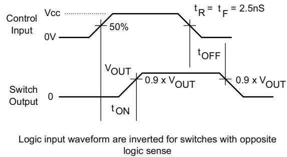
Figure 1. Turn-On/Turn-Off Timing
