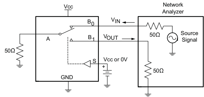
Figure 6. Crosstalk
