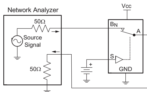
Figure 10. Bandwidth
