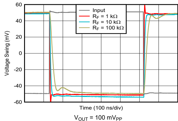
Figure 6-10. Small-Signal Transient Response
