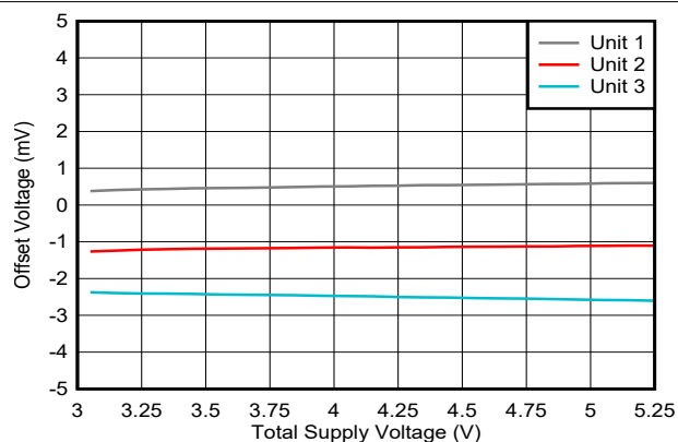
Figure 6-20. Offset Voltage vs Supply Voltage
