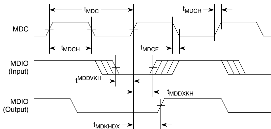
Figure 20. MII Management Interface Timing Diagram
