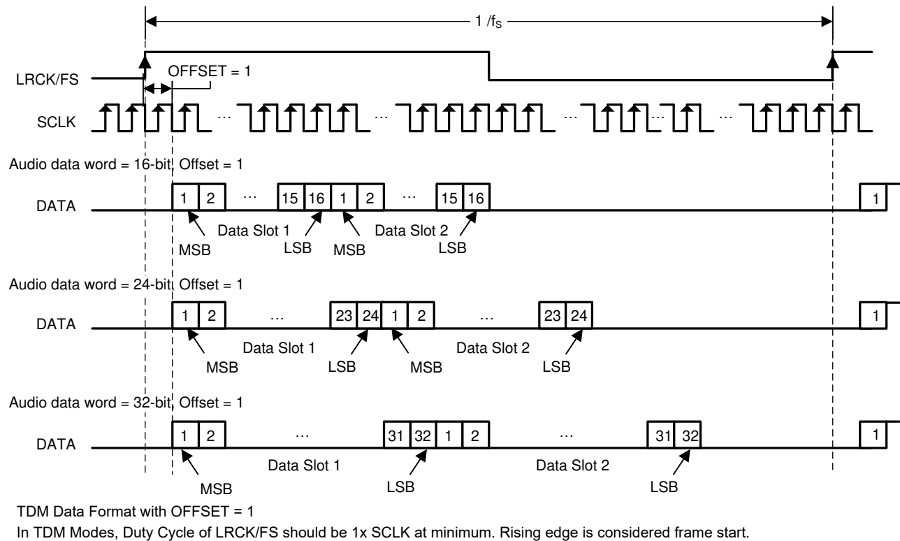
Figure 8-6. TDM 2 Audio Data Format
