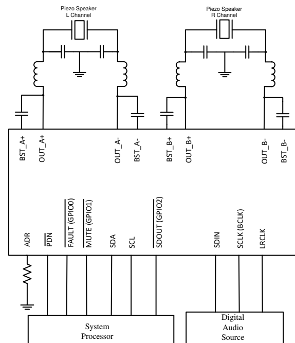
Simplified Schematic
