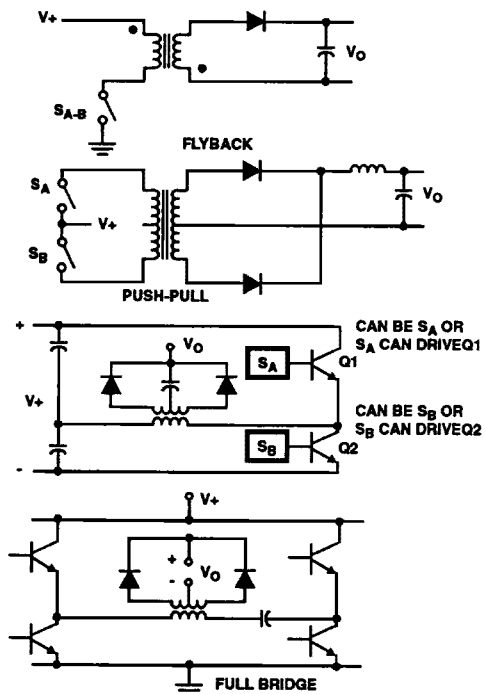
FIGURE 17. TRANSFORMER-COUPLED OUTPUTS
