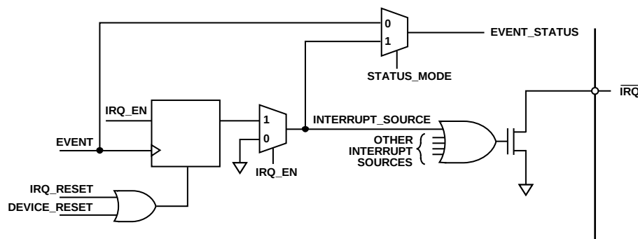
Figure 87. Simplified Schematic of \overline{IRQx} Circuitry
