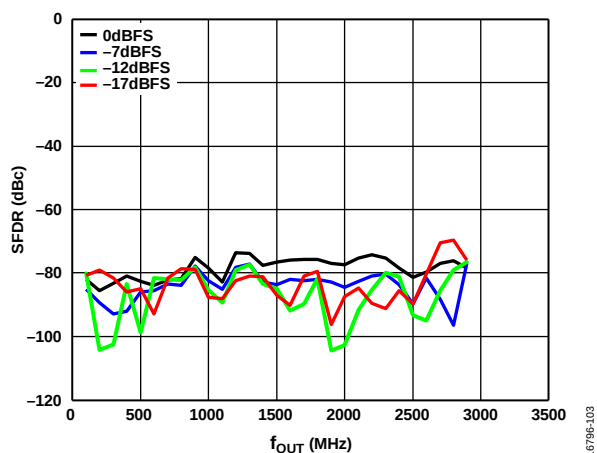
Figure 3. Second Harmonic (SFDR) vs. f_{OUT} over Digital Scale (Mode 0), 6 GHz DAC Sample Rate, Channel Interpolation 2 \times , Main Interpolation 8 \times
