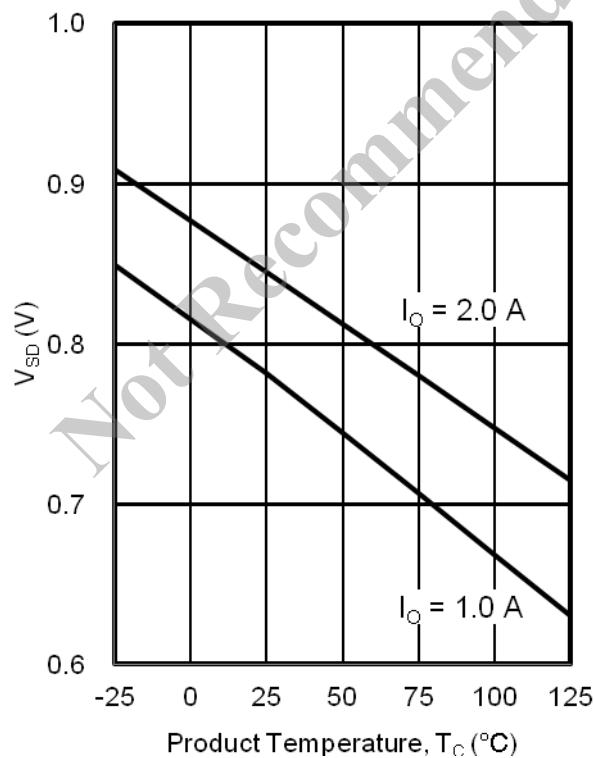
SLA7072MS / SLA7077MS
