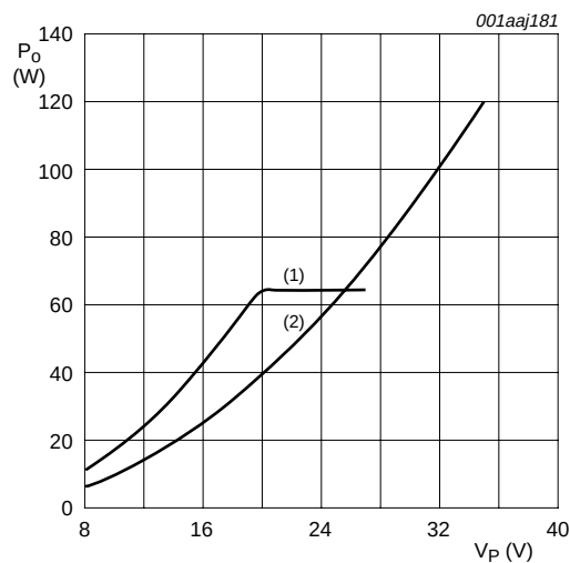
THD = 0.5 %. R DSon = 0.2 Ω (at T j = 100 °C), R s = 0.05 Ω, t w(min) = 190 ns and I O(ocp) = 8 A (minimum). (1) R L = 2 Ω. (2) R L = 4 Ω.
