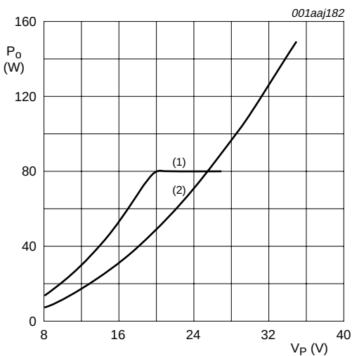
THD = 10 %. R DSon = 0.2 Ω (at T j = 100 °C), R s = 0.05 Ω, t w(min) = 190 ns and I O(ocp) = 8 A (minimum). (1) R L = 2 Ω. (2) R L = 4 Ω.
