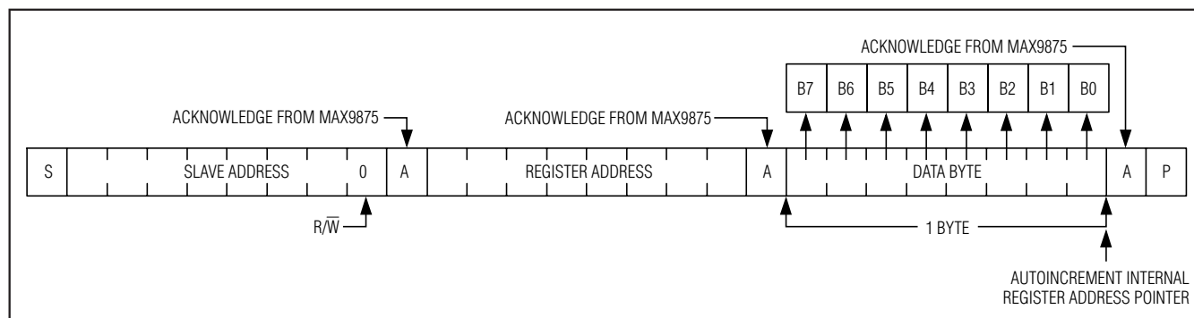
Figure 9. Writing One Byte of Data to the MAX9875
