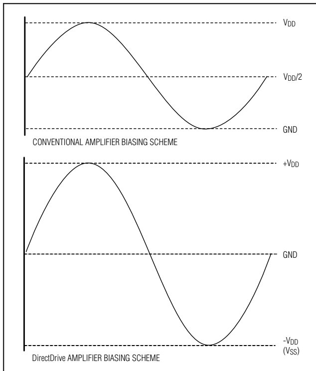
Figure 5. Traditional Amplifier Output vs. MAX9875 DirectDrive Output
