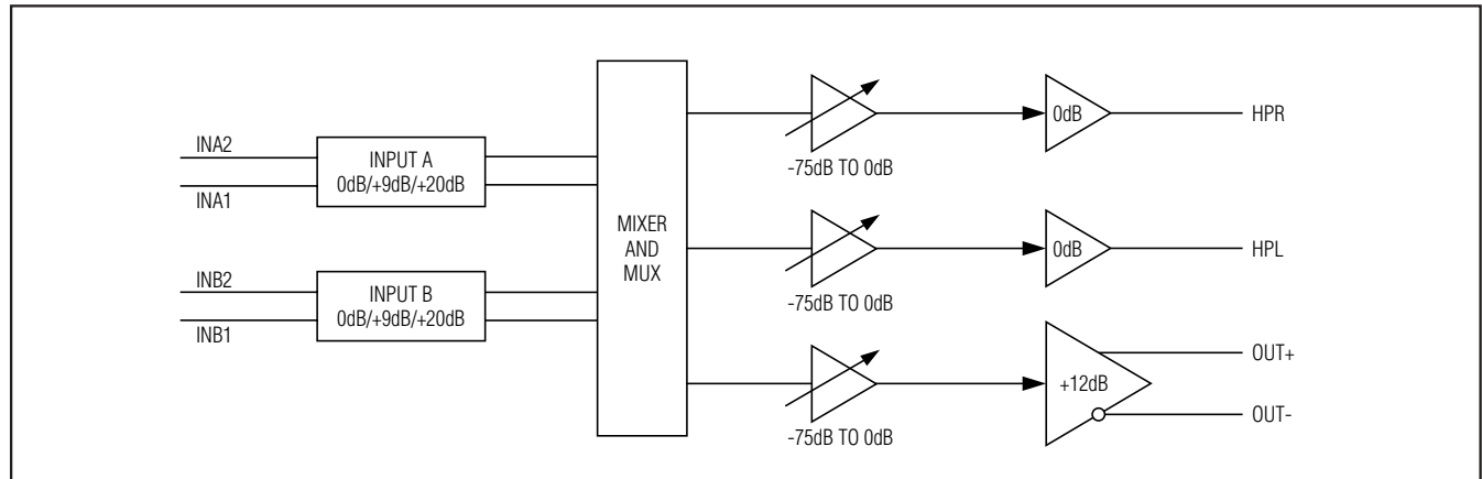
Figure 1. Signal Path
