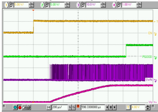
Top: EN1, CH1 Enable Signal, (5V/div) Middle 1: PGOOD1, CH1 Power Good Signal, (5V/div) Middle 2: SWN1, CH1 Switching Node Voltage, (10V/div) Bottom: Vo1, CH1 Output Voltage, (1V/div) Time: 200μs/div
