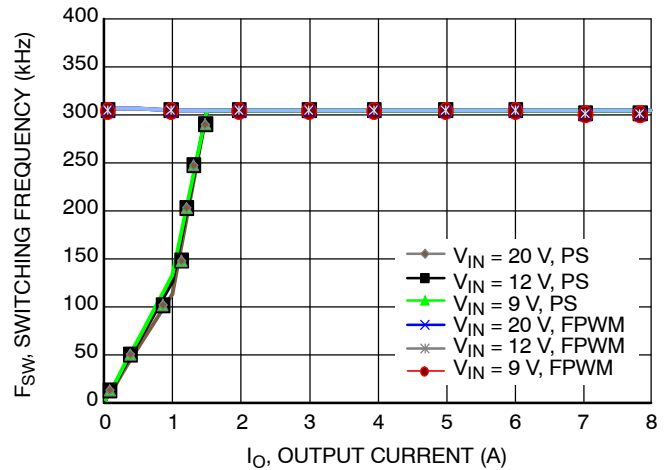
Figure 13. Switching Frequency vs. Output Current ( V_O = 1.05 V)
