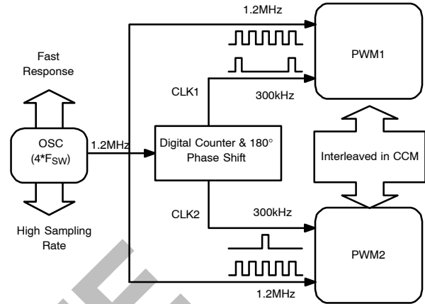
Figure 28. Internal Clocks in the NCP5215 as F_{sw} = 300 \text{ kHz}
