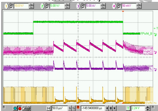
Top: FPWM#, FPWM# Signal, (5V/div) Middle 1: Vo1, CH1 Output Voltage Ripple, (50mV/div) Middle 2: iL1, CH1 Inductor Current, (5A/div) Bottom: SWN1, CH1 Switching Node Voltage, (10V/div) Time: 50μs/div
