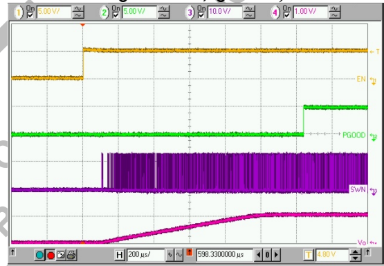
Top: EN2, CH2 Enable Signal, (5V/div) Middle 1: PGOOD2, CH2 Power Good Signal, (5V/div) Middle 2: SWN2, CH2 Switching Node Voltage, (10V/div) Bottom: Vo2, CH2 Output Voltage, (1V/div) Time: 200μs/div
