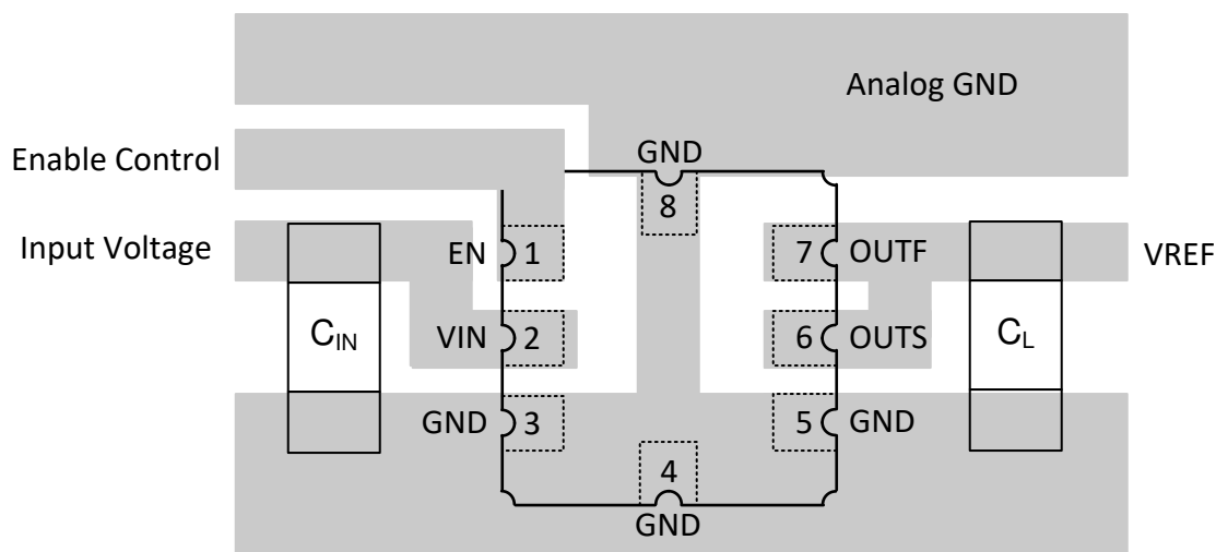
Figure 12-1. Layout Example
