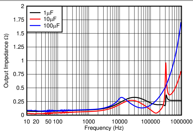
Figure 7-10. Output Impedance
