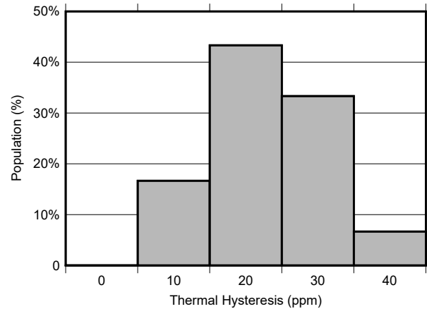
Figure 8-5. REF7012 Thermal Hysteresis Distribution (-40°C to 125°C)
