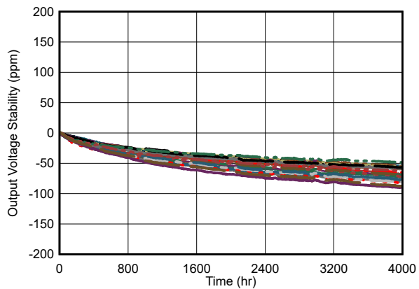
Figure 7-20. Long-Term Stability (First 4000 Hours)
