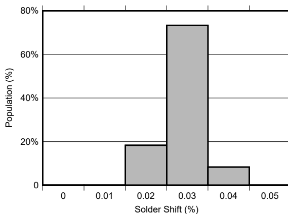
Figure 8-2. Solder Shift
