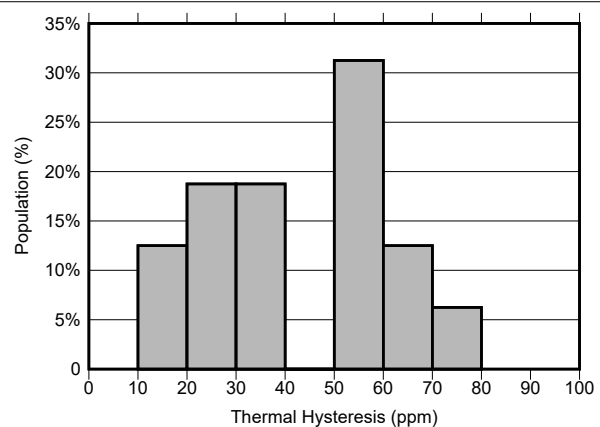
Figure 7-18. REF7025 FKH Thermal Hysteresis Distribution (0°C to 70°C)
