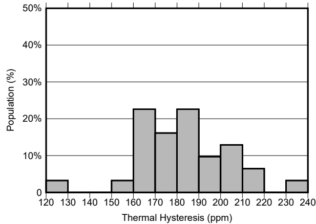
Figure 8-4. REF7025 Thermal Hysteresis Distribution (-40°C to 125°C)
