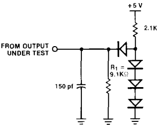
Figure 14. Test Load 1
