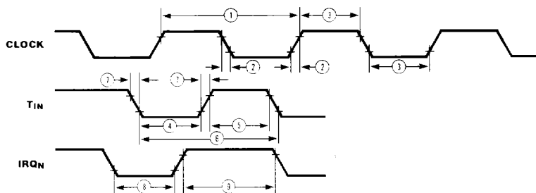
Figure 16. Additional Timing
